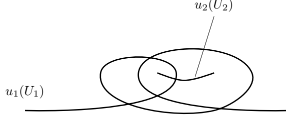
FIGURE 4. Interpenetrating curves with \deg(\hat{u}_1, \hat{U}_1, u_2(x)) \neq 0 for all extensions \hat{u}_1 of u_1 and x \in U_2 .
