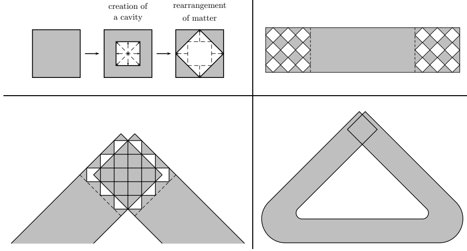
FIGURE 1. The pathological example by Müller and Spector.
