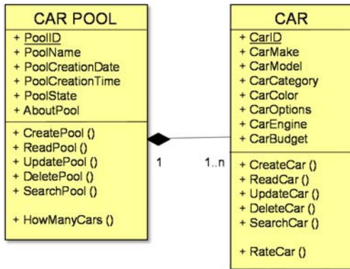
Figure 3. A partial domain model for car rental.
