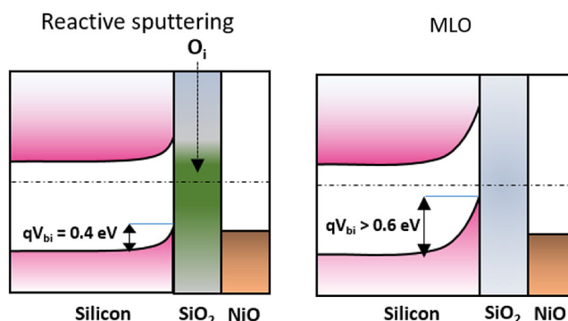
Figure 8. Band-diagram representing the \text{Si}/\text{SiO}_2/\text{NiO} junction when NiO is deposited by reactive sputtering (left) or by metal-layer-oxidation (right). The silicon band-bending is pinned at 0.4 eV for reactively sputtered NiO due to the presence of oxygen interstitial ( \text{O}_i ), while it might exceed 0.6 eV if NiO is prepared by the MLO method.
