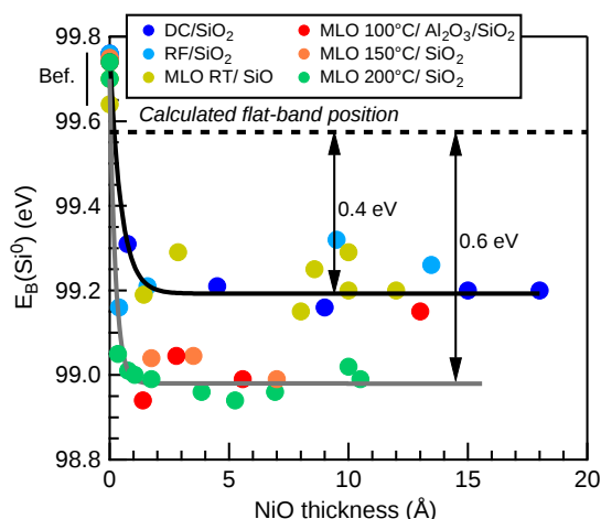
Figure 7. Binding energy of \text{Si}^0 peak during interface formation of n\text{-Si}/\text{SiO}_2 substrates with differently deposited NiO in dependence on NiO film thickness. The \text{Si}^0 binding energies of the uncovered, hydrogen passivated samples are slightly above the calculated flat-band position. It suggests that negative charges accumulate at the interface. The label Bef. stands for Before and aim at emphasizing the position of the \text{Si}^0 before the deposition of NiO.
