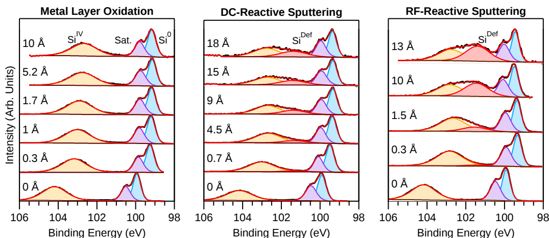
Figure 4. Si 2p spectra measured by XPS during the interface experiments with NiO on Si/SiO 2 substrates. Three deposition method have been evaluated: MLO, DC reactive sputtering, and RF reactive sputtering. The spectra are normalized to the Si 0 intensity for better comparison of the evolution of the peak shapes.
