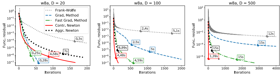
Figure 2: Training logistic regression, w8a ( M = 49749, n = 300 ).
