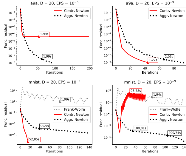
Figure 5: Influence of the parameter of inner accuracy.
