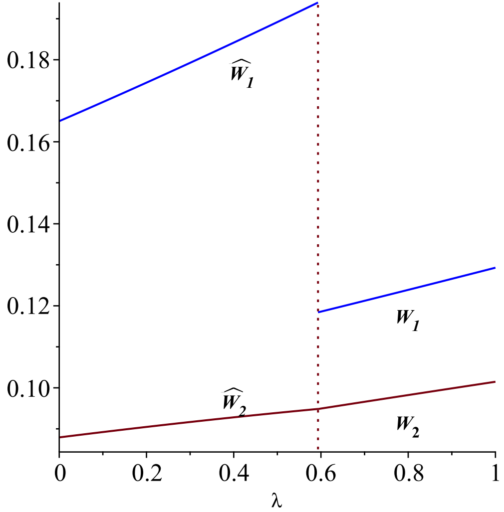
Figure 1: The minimum tax breaks the tax compliance agreement when the minimum tax is sufficiently high: \rho = -1 , \epsilon = 0.22 , \widehat{W}_i = W_i(\hat{e}^M) and W_i = W_i(e^M) .
