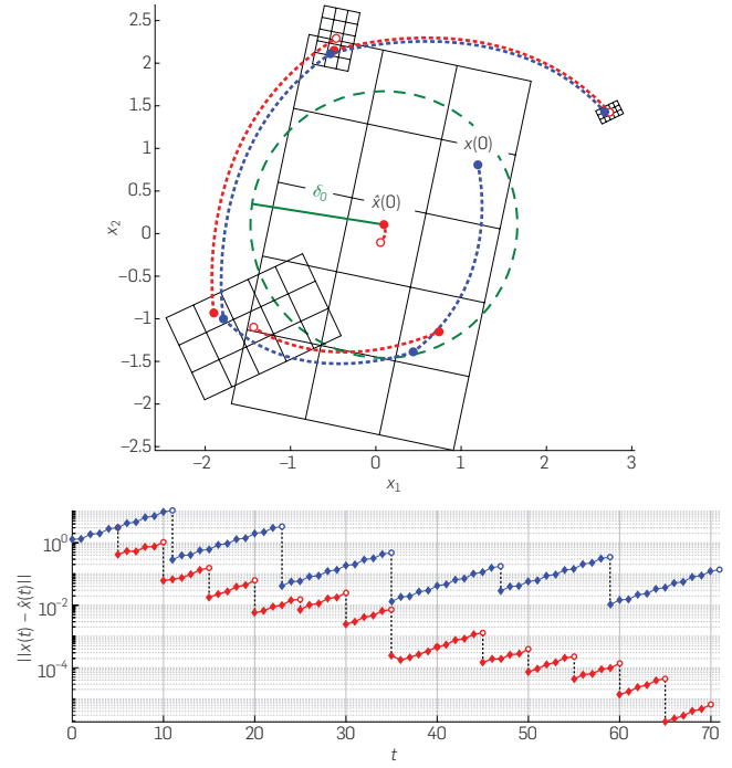
Figure 5. Top: Evolution of x(t) and \hat{x}(t) for a sample execution of the coder-decoder with data rate R = 4 . Bottom: Evolution of the estimation error \|x(t) - \hat{x}(t)\| for sample executions of the coder-decoder with data rates R = 0.8 (red) and R = 0.5 (blue). The vertical gray lines indicate the transmission times T_j (in general, the error decreases at these times because the decoder receives a new symbol).
