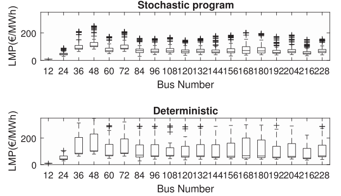
Fig. 6. The locational marginal prices of the stochastic and deterministic dispatch policies. The boxes include the observations within the 25% and 75% quantiles, the crosses correspond to outliers.
