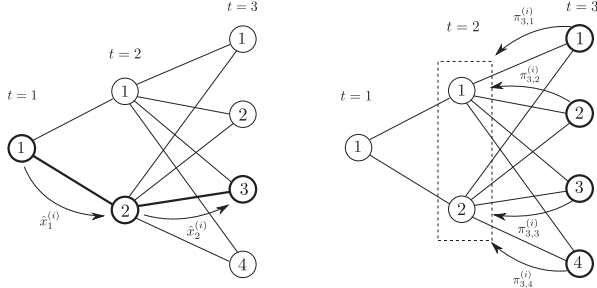
Fig. 7. An illustration of the lattice used in the SDDP algorithm.
