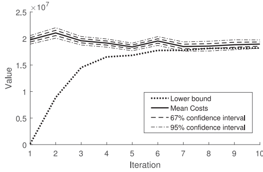
Fig. 3. The evolution of lower and upper bounds of the SDDP algorithm.
