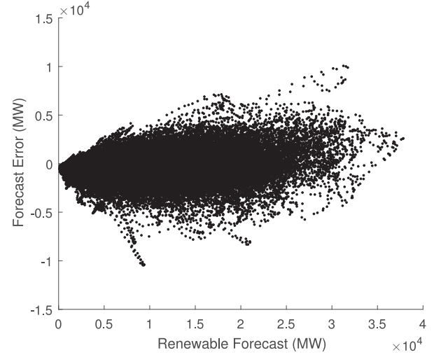
Fig. 1. The scatter plot of wind and solar production day-ahead forecasts versus historical forecast error in Germany for 2013 and 2014.
