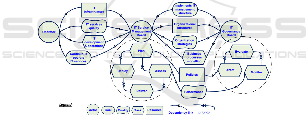
Figure 3: GI-Tropos Strategic Rationale model.
