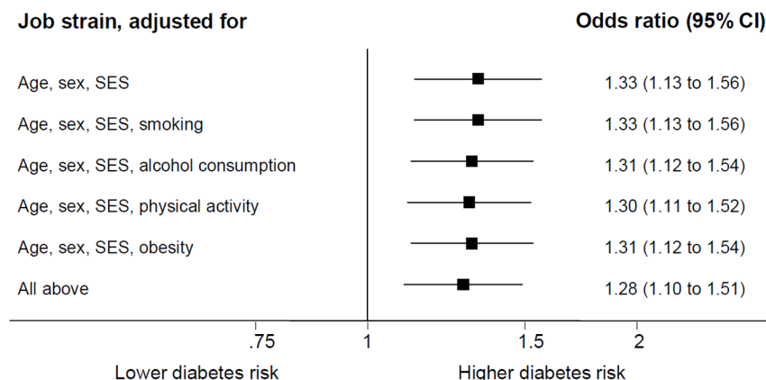
Figure 1. Adjusted Odds Ratios (95% CI) for the Association Between Job Strain and Diabetes (N = 44,818 in All Models), the IPD-Work Consortium, 1984–2003.
