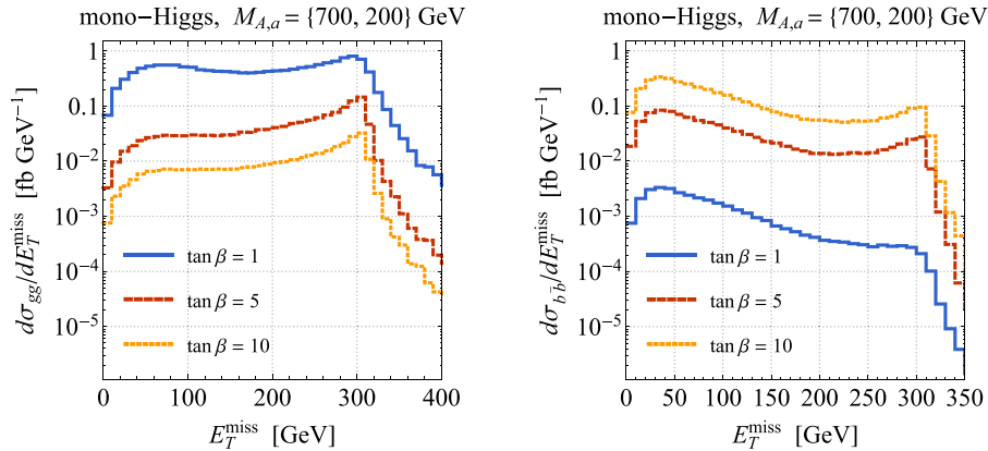
Fig. 14. E_T^{\text{miss}} distributions for mono-Higgs production in gg-fusion (left panel) and b\bar{b} -fusion (right panel) in the 2HDM+a model. The displayed results correspond to pp collisions at 13 TeV and different choices of \tan \beta . The parameters not detailed in the plots are set to (17) using M_H = M_A = M_{H^\pm} = 700 GeV and M_a = 200 GeV.
