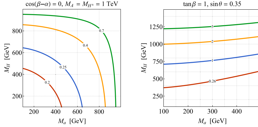
Fig. 4. Left: Values of M_a and M_H allowed by EW precision constraints assuming \cos(\beta - \alpha) = 0 , M_A = M_{H^\pm} = 1 TeV and four different values of \sin \theta , as indicated by the contour labels. The parameter space below and to the left of the contours is excluded. Right: Constraints in the M_a - M_H plane following from the BFB requirement. The results shown correspond to \tan \beta = 1 , \sin \theta = 0.35 and degenerate heavy spin-0 boson masses M_H = M_A = M_{H^\pm} . The region above each contour is excluded for the indicated value of the quartic coupling \lambda_3 .
