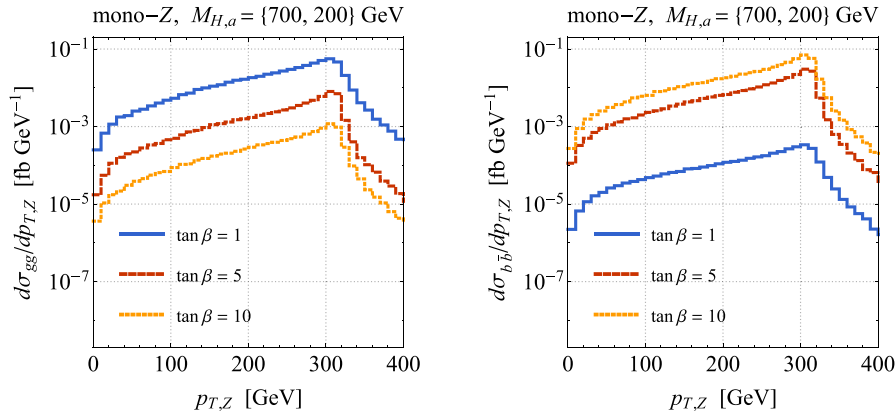
Fig. 15. p_{T,Z} distributions for mono-Z production in gg-fusion (left panel) and b\bar{b} -fusion (right panel) in the 2HDM+a model. The predictions shown correspond to pp collisions at 13 TeV and the same choices of parameters as in Fig. 14 are employed.
