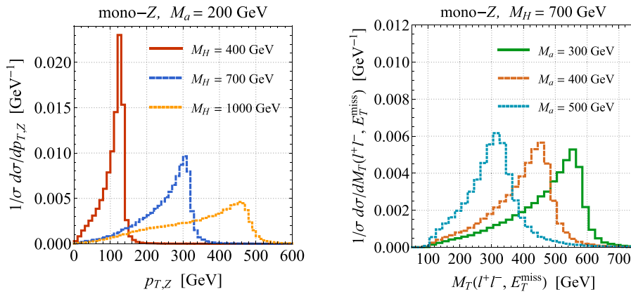
Fig. 8. Normalised p_{T,Z} (left panel) and M_T(\ell^+ \ell^-, E_T^{\text{miss}}) (right panel) distributions for Z + E_T^{\text{miss}} production followed by Z \rightarrow \ell^+ \ell^- . The predictions shown have been obtained for the 2HDM+a benchmark parameter choices given in (17) and employ different values of M_H and M_a as indicated in the legends.
