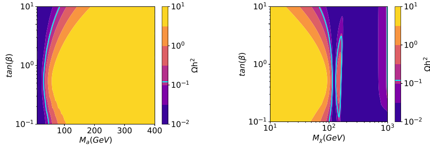
Fig. 29. Predicted DM relic density in the 2HDM+a model in the M_a - \tan\beta (left panel) and m_\chi - \tan\beta (right panel) plane, respectively. In the left (right) panel, m_\chi = 10 GeV ( m_a = 250 GeV) is employed as well as M_H = M_A = M_{H^\pm} = 600 GeV. The colour coding is identical to Fig. 27.
