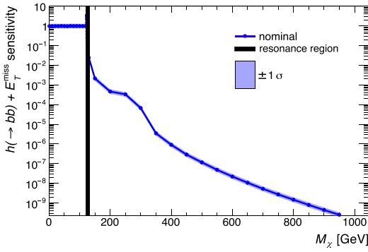
Fig. C.34. Estimated sensitivities of the h(b\bar{b}) + E_T^{\text{miss}} channel as a function of m_\chi . The results shown correspond to M_H = M_A = M_{H^\pm} = 600 GeV, M_a = 250 GeV and the parameter choices made in (17). The colour coding resembles that used in Fig. C.33. It is recommended to stay at least 1 GeV away from the region where M_a = 2m_\chi to avoid numerical effects from the resonance in the generation.
