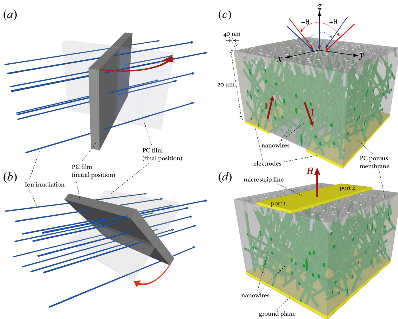
FIG. 1. Schematics of the track etching process (a) for the first irradiation step under an angular range of \pm 45^\circ relative to the out-of-plane direction and (b) for the second irradiation step after in-plane PC membrane rotation by 90^\circ and again under the same angular range relative to the OOP direction. (c) Schematic representation of a 3D PC template prepared by the successive irradiation steps of (a) and (b), featuring cylindrical nanopores with a mean diameter of 40 nm and partially filled with magnetic CNWs. An electrode design for two-probe electrical measurement obtained by local etching of the Cu cathode is also shown. (d) Schematic of a stripline transmission line for FMR measurement fabricated using similar partially filled membrane.
