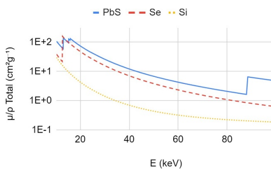
Figure 21. Mass x-ray attenuation coefficient for PbS, Se, and Si.
