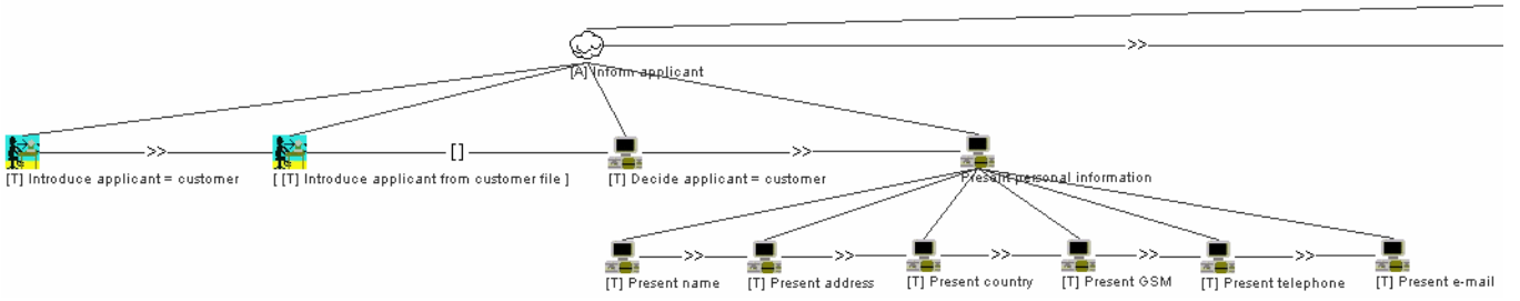
Figure 4. Task model.
