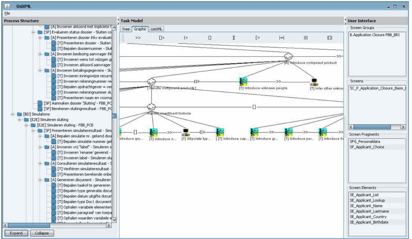
Figure 7. Traceability Tool
