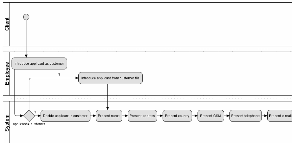
Figure 3. Business process.
