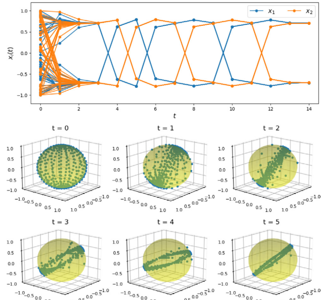
Fig. 3. Top: Normalized trajectories of the SLS from Example 4, starting from different initial conditions and for a random s.s. \sigma . Bottom: Normalized trajectories of a 2-dominant SLS starting from different initial conditions and for a random s.s. \sigma . Each dot represents the projection on the sphere of a trajectory x(\cdot) at times t = 0, 1, \dots, 5 .
