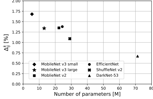
Fig. 7. Complexity/accuracy trade-off for 6 different KDN backbones. The common trend is that larger networks achieve lower errors on keypoint locations.
