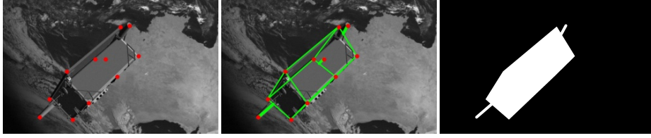
Fig. 5. Computation of pseudo ground-truth segmentation masks. left: Keypoint coordinates may be computed by projecting the spacecraft model on the image plane according to its relative pose. middle: Body Edges are directly computed from the body keypoints while antennas may be approximated as a straight line segment between their corresponding keypoint and their basis on the spacecraft body. right: The approximate segmentation mask can be recovered by filling in the body parts.
