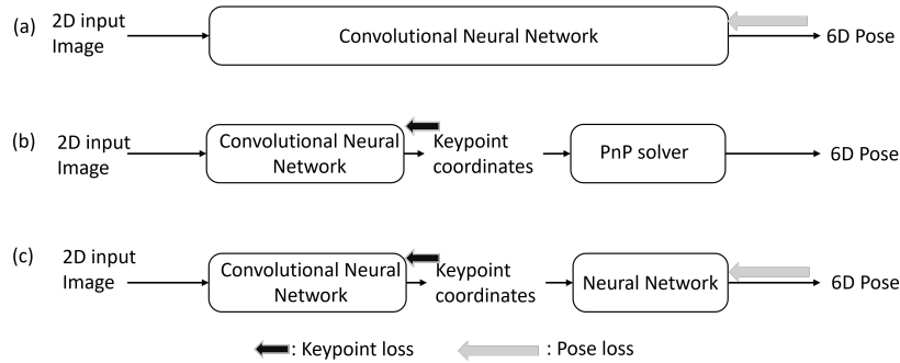
Fig. 1. Overview of the existing methods to estimate a spacecraft’s pose. (a) Direct methods use a convolutional neural network to directly predict the target 6D pose. (b) Keypoints-based methods exploit a convolutional neural network to predict pre-defined keypoint coordinates which are then used to recover the pose through a Perspective-n-Point (PnP) solver. (c) Our solution combines both methods as it relies on a first, convolutional, neural network to extract the coordinates of pre-defined keypoints and a neural network to predict pose from those coordinates. The solution is therefore both keypoints-based and end-to-end trainable.
