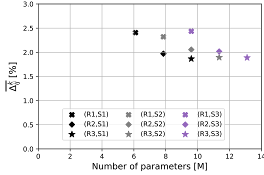
Fig. 8. Complexity/accuracy trade-off for a KDN based on MobileNet v3 large with 9 different heads architectures. Each setting is labelled (RX,SY) where X is the number of blocks per stage in the regression head and Y is the number of blocks per stage in the segmentation one. Reducing the complexity of the regression head increases the error on the keypoints. The complexity of the segmentation head has a negligible impact on the predictions accuracy.
