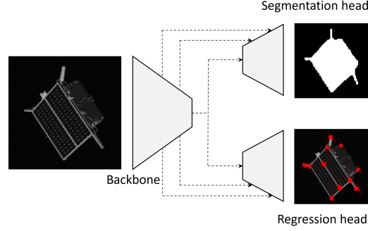
Fig. 3. Architecture of the Keypoint Detection Network [15]. It is made of a backbone and two decoding heads. The first head performs a segmentation of the spacecraft while the second head regresses candidate locations of some pre-defined keypoints. Dashed lines represent skip connections [25].
