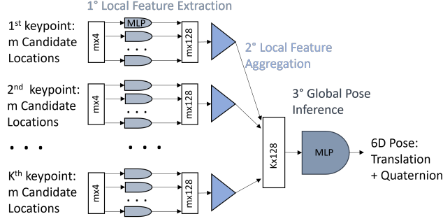
Fig. 6. Architecture of the Pose Inference Network [14]. Local features are extracted from every candidate location through a MLP which weights are shared across all candidates and all keypoints. Those local features are then aggregated per keypoint into a single representation. Finally, the final pose is inferred through a MLP fed by those keypoint representations.
