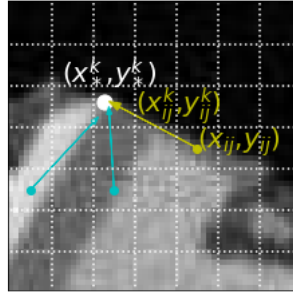
Fig. 4. Illustration of some offsets predicted by the KDN. (x_*, y_*)^k are the ground-truth coordinates of the keypoint k . (x_{ij}, y_{ij})^k are the coordinates of the center of a patch. This patch predicts an offset (x_{ij}^k, y_{ij}^k) pointing toward keypoint k .
