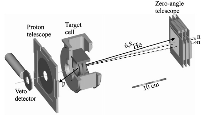
Fig. 1. Experimental setup and kinematical diagram.
