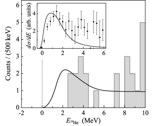
Fig. 7. Missing mass spectrum of ^{10}\text{He} compared to the predictions of Ref. [11] for the ^{10}\text{He} g.s. with the [p_{1/2}^2] structure. The inset shows the experimental data of Ref. [4] compared to the theoretical spectrum obtained with the same Hamiltonian as in the main panel but for the different reaction mechanism.
