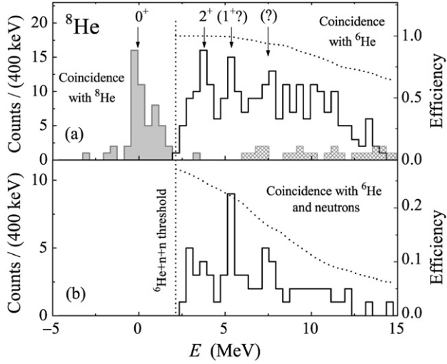
Fig. 2. Missing mass spectrum of ^8\text{He} . (a) The p - ^8\text{He} and p - ^6\text{He} coincidence data were used to obtain the ground state peak and the excited state spectrum, respectively. The hatched histogram demonstrates the measured background contribution: the empty target run results are shown, processed in the same way as the real data and scaled to the beam current integral of the working run. (b) Spectrum built for the ^8\text{He} excited states from the p - ^6\text{He} - n coincidence data. The efficiencies of the p - ^6\text{He} and p - ^6\text{He} - n coincidence registration are shown by dotted curves (see the right axes in both panels).
