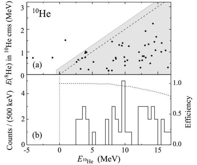
Fig. 3. Scatter plot showing the ^8\text{He} energy observed in the ^{10}\text{He} CMS frame versus the ^{10}\text{He} missing mass energy. (b) Missing mass spectrum of ^{10}\text{He} . The p - ^8\text{He} coincidence efficiency is shown by dotted curve (see right axis).
