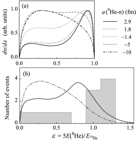
Fig. 8. Energy distribution of {}^8\text{He} in the {}^{10}\text{He} CMS frame. (a) Calculated in Ref. [11] for different interactions in the {}^8\text{He} - n channel. The corresponding scattering lengths are shown in the legend; positive a values correspond to repulsive interactions. Solid curve corresponds to the theoretical missing mass spectrum given in Fig. 7 ( {}^{10}\text{He} g.s. with [p_{1/2}^2] structure). (b) E({}^8\text{He}) distribution observed in the present work for the 3 MeV group of events is shown as a gray histogram. Theoretical curves are the same as in panel (a) convoluted by the MC procedure with the experimental resolution.
