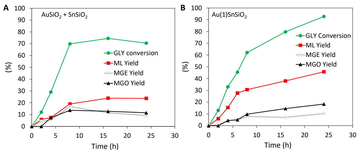
Figure 4: transformation glycerol (GLY) to methyl lactate (ML), methyl glycerate (MGE) and methyl glycolate (MGO) with (A) the mechanical mixture of AuSiO 2 and SnSiO 2 (200 mg of each catalyst), (B) the bifunctional catalyst Au(1)SnSiO 2 (200 mg). Reaction conditions: T = 140°C, p air = 30 bar, 0.25 M glycerol in methanol, and GLY/gold-based catalyst ratio = 2.3 (w/w).
