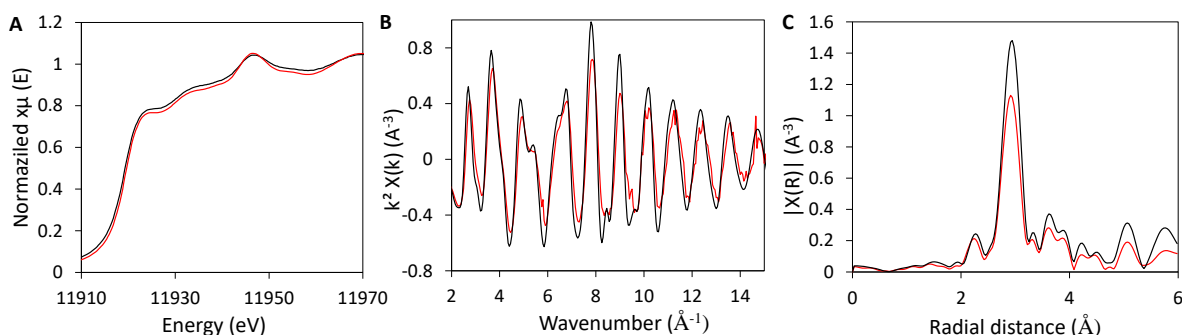
Figure 6: (A) normalized XANES spectra, (B) k^2 \chi(k) EXAFS interference functions and (C) corresponding FTs moduli (phase shift corrected) of Au(1)SnSiO 2 (red curves) and Au foil (black curves). Note that, similarly, the Sn signal was not affected by the presence of Au.
