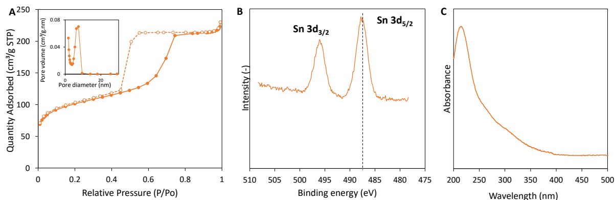
Figure 3: Nitrogen adsorption (plain symbols) and desorption (empty symbols) isotherms of SnSiO 2 . Insert show BJH pore size distribution analysis obtained from the adsorption isotherm. (B) XPS spectra of the Sn3d region with indication (dotted line) of the theoretical binding energy of Sn3d 5/2 in Sn 4+ state (487.2 eV) 61 . In (C) Diffuse reflectance UV/Vis spectrum of SnSiO 2 .
