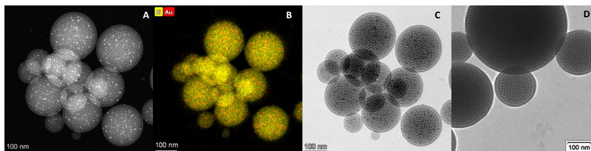
Figure 1: Transmission electron microscope analysis of (A,B,C) AuSiO 2 and (D) SnSiO 2 . Respectively from left to right: HAADF, STEM-EDX, STEM.
