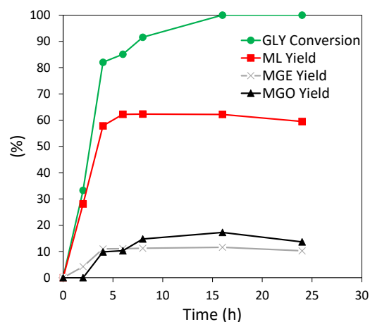
Figure 8: transformation glycerol (GLY) to methyl lactate (ML), methyl glycerate (MGE) and methyl glycolate (MGO) with Au(1)SnSiO 2 . Reaction conditions: T = 160°C, p air = 15 bar, 0.125 M glycerol in methanol, and GLY/Catalyst ratio = 1.15 (w/w).
