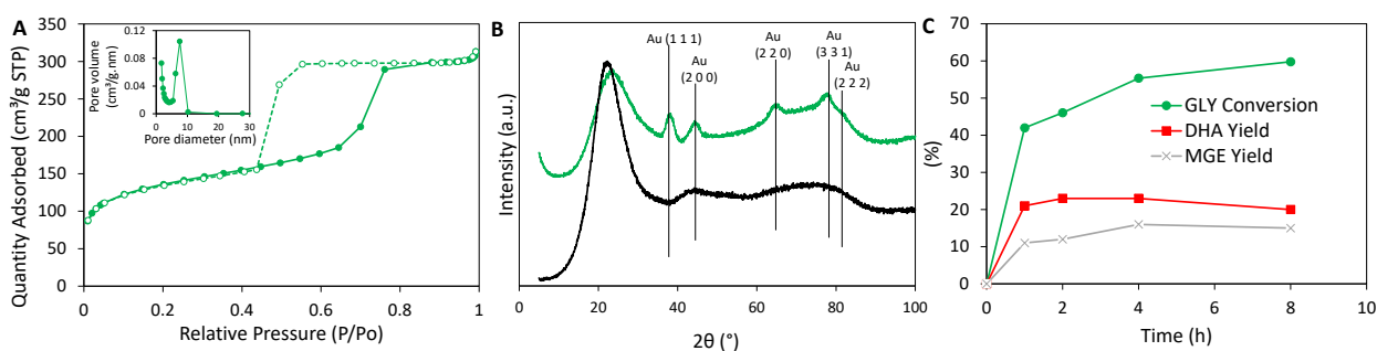
Figure 2: (A) Nitrogen adsorption (plain symbols) and desorption (empty symbols) isotherms of AuSiO 2 . Insert shows BJH pore size distribution analysis obtained from the adsorption isotherm. (B) XRD diffractogram of fresh AuSiO 2 (black) and calcined AuSiO 2 (green) (the detected metallic Au phase corresponds to JCPDS 65-2870). (C) Kinetic study of the oxidation glycerol (GLY) to dihydroxyacetone (DHA) and methyl glycerate (MGE) with AuSiO 2 . Reaction conditions: T = 140^{\circ}\text{C} , p_{\text{air}} = 30 bar, 0.25 M glycerol in methanol, and GLY/Catalyst ratio = 2.3 (w/w).
