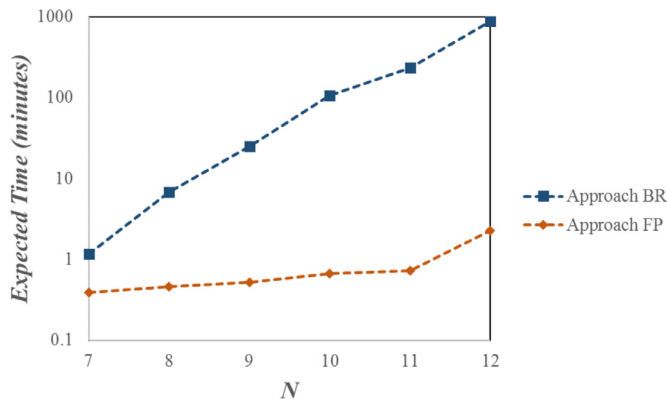
Fig. 3. Estimated computational time for computing payoff matrices for long horizons lengths.
