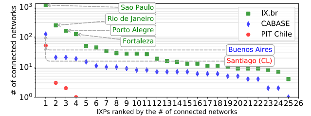
Figure 2: Number of connected networks to regional IXPs in IX.br, CABASE and PIT Chile in July 2019.
