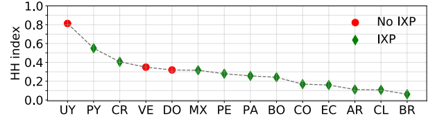
Figure 5: Herfindahl-Hirschman Index to determine originated address space concentration in countries that have been delegated more than 1M IP addresses.
