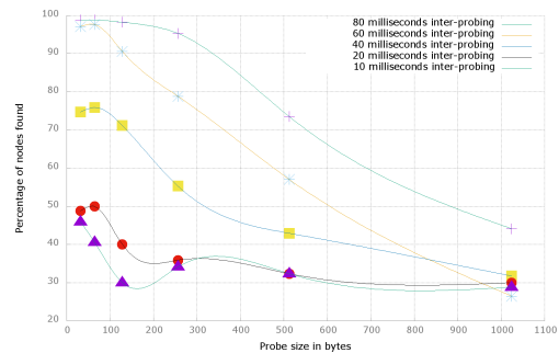
Fig. 12. Number of IEEE 802.15.4 nodes found; normal background.
