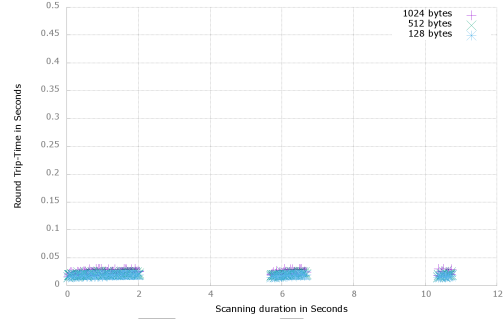
Fig. 5. RTT for IEEE 802.11; normal background, T = 20 ms.
