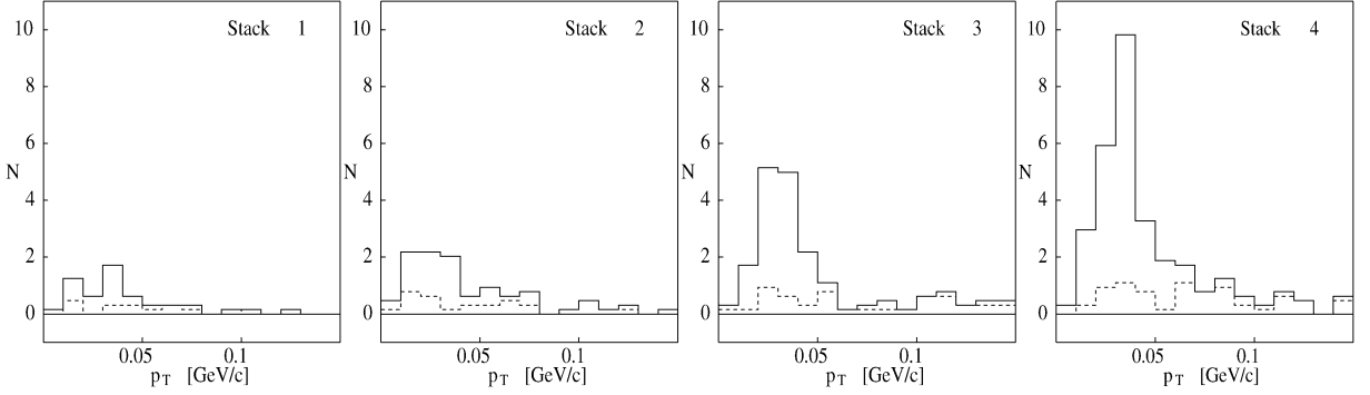
Fig. 1. Simulated transverse-momentum distribution of charged hadrons from the primary vertex with respect to the D^0 direction. The meaning of the histograms is explained in the text. The four panels show the simulation for the four emulsion stacks, stack one being the most upstream stack.
