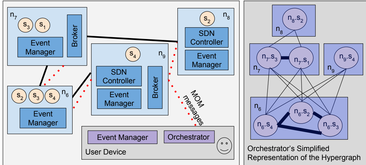
Figure 7.2: An Évora deployment: Edge Nodes and the User Device
