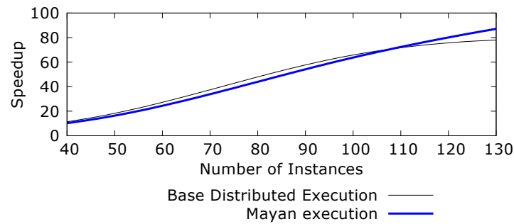
Figure 6.7: Speedup of distributed data cleaning and consolidation workflow
