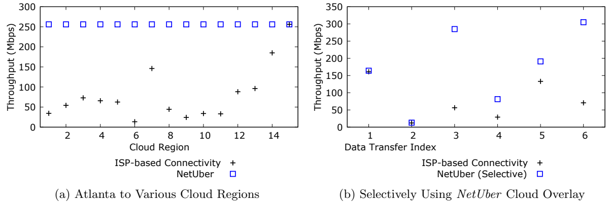
Figure 4.6: Throughput of NetUber with ISP-based cloud connect
