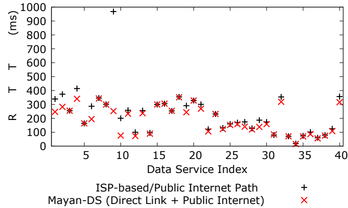
Figure 10.3: Ping times of Mayan-DS against the Public Internet-based Connectivity
