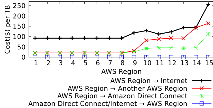
Figure 4.2: Data Transfer Cost for AWS
