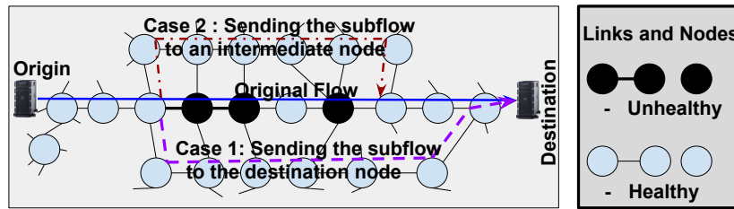
Figure 5.1: Subflows and Alternative Execution Paths
