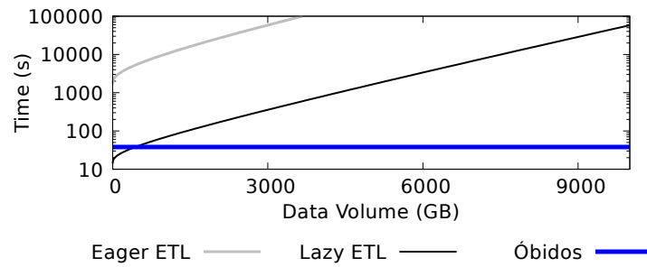
Figure 9.7: Load time from the remote data sources
