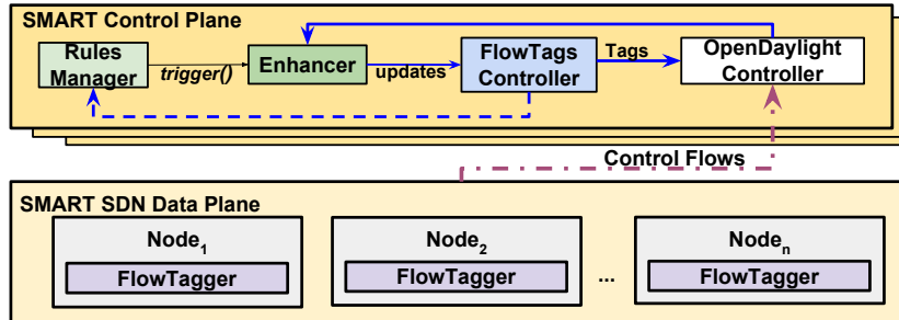
Figure 5.3: SMART Architecture
