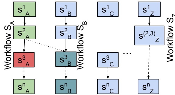
Figure 6.1: A sample representation of multiple alternative workflow executions.
