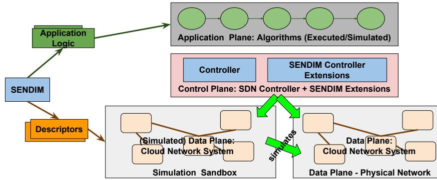
Figure 3.1: Separation of the Application Logic From the Execution Environment
