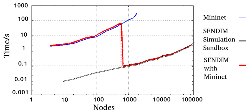
Figure 3.7: Network Construction with Mininet and SENDIM Simulation Sandbox
