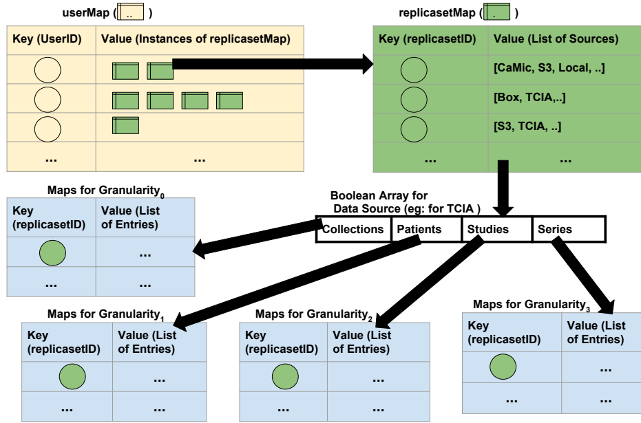
Figure 9.4: Data Structures of the Replicaset Holder
