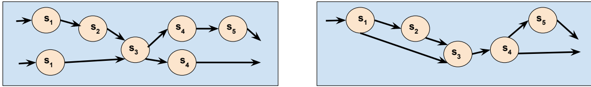
Figure 6.2: Parallel Execution Alternatives of a Service Composition Workflow
