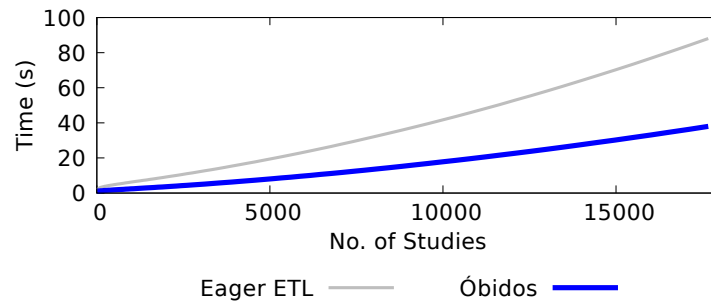
Figure 9.8: Query completion time for the integrated data repository
