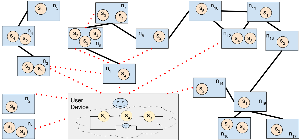
Figure 7.1: A User-Defined NSC Among the Edge Nodes
