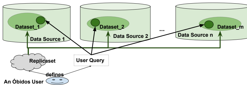
Figure 9.2: Narrowing down the search space with user-defined replicaset
