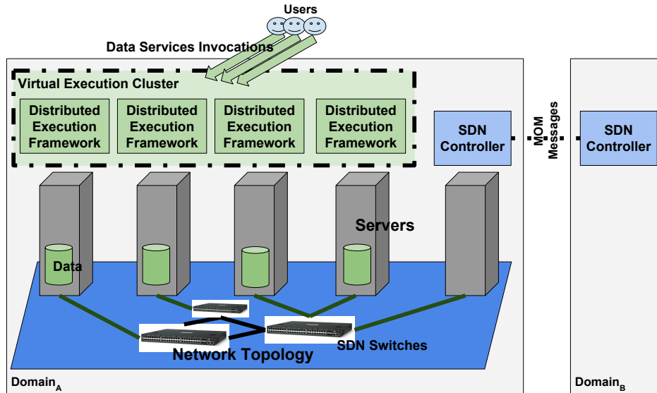
Figure 10.1: A Sample Mayan-DS Deployment
