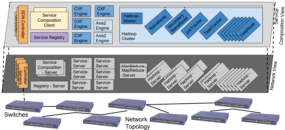
Figure 6.4: Three-Dimensional View of Mayan : Hosts, Network Topology, and Services
