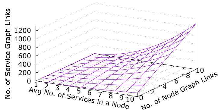
Figure 7.3: Representation of the service graph from the node graph
