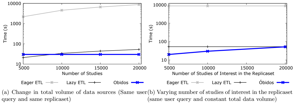
Figure 9.6: Data load time
