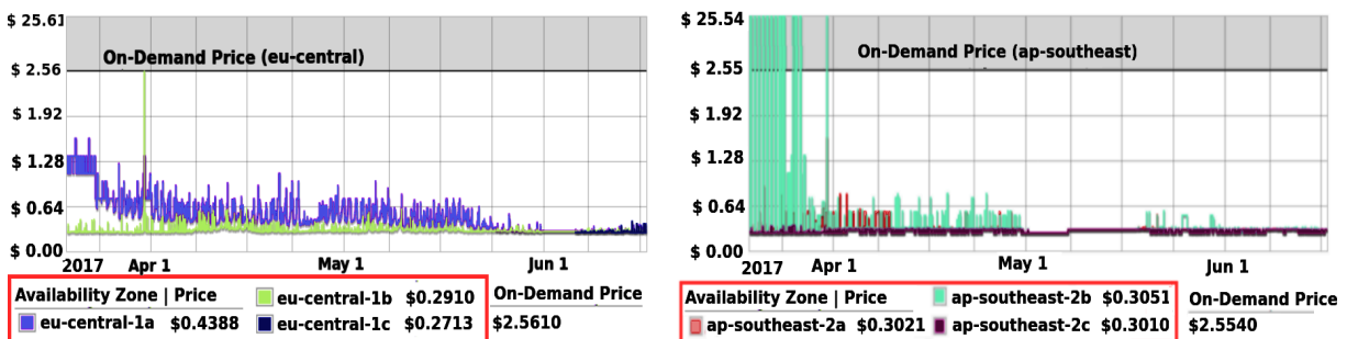
Figure 4.1: Linux r4.xlarge Spot Instance Price in Frankfurt and Sydney, April - June 2017
