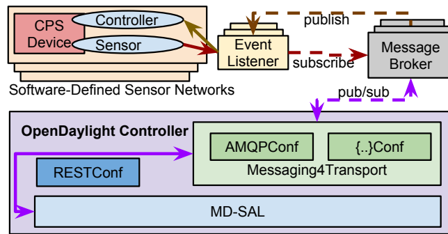
Figure 8.3: Network Layer - Higher Level View
