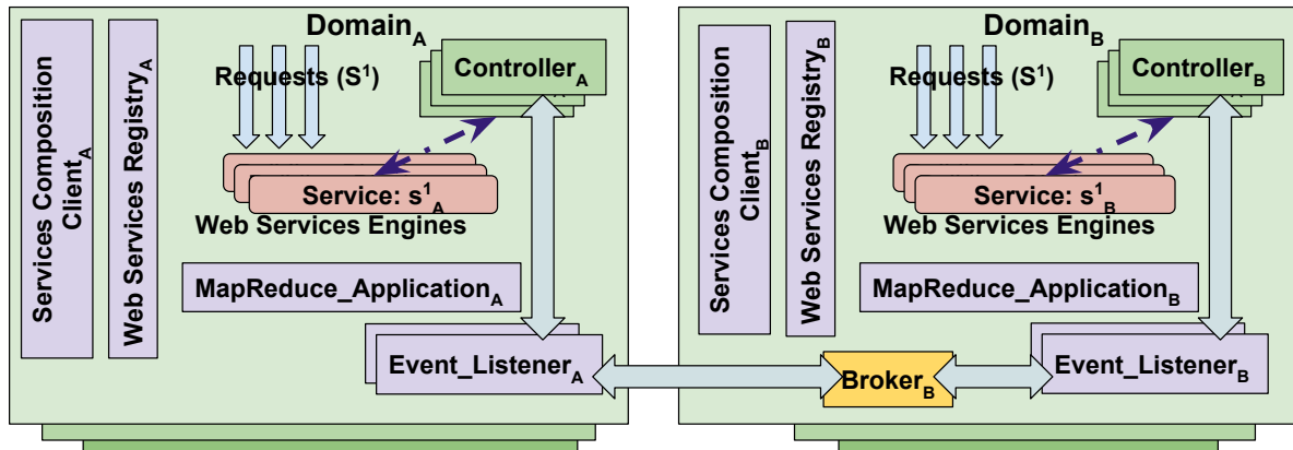
Figure 6.3: Inter-Domain Service Compositions with Mayan Controller Farm
