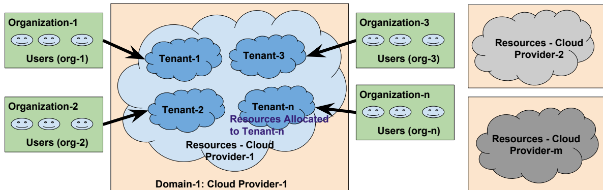
Figure 1.1: Multitenancy and the Tenant Users of a Cloud Environment
