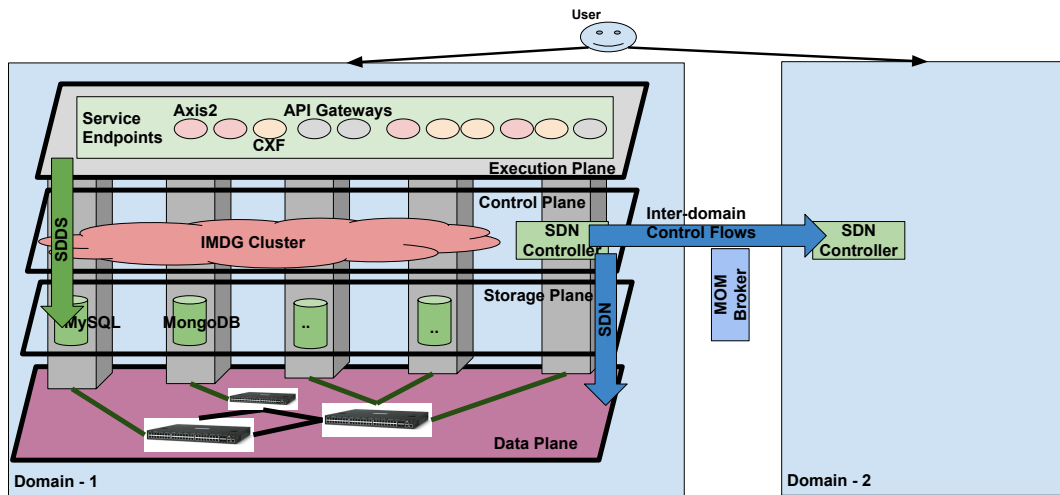
Figure 10.2: A Three-Dimensional View of the Mayan-DS Implementation
