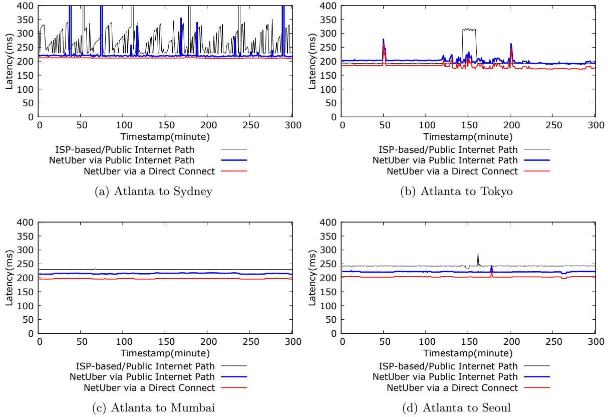
Figure 4.7: Latency (RTT) variations of NetUber and the ISP-based Internet paths
