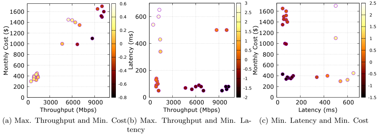
Figure 7.4: Évora policies with two attributes of equal weight.
