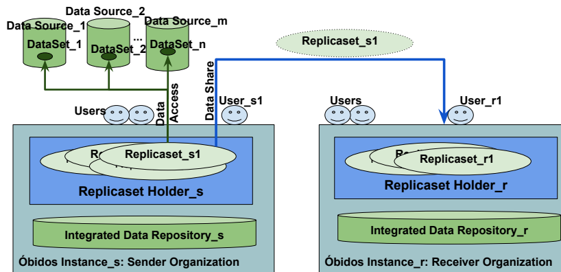
Figure 9.3: Data Sharing with Óbidos
