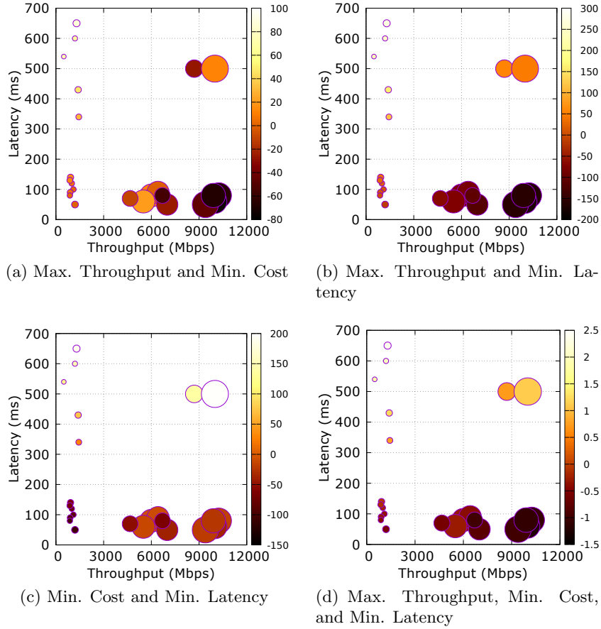
Figure 7.6: Évora policies considering three attributes with prominence to two or all of the three attributes. The radius of the circles represents the cost.
