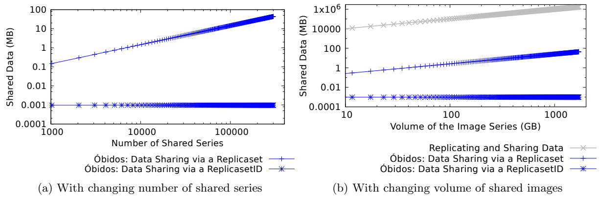
Figure 9.9: Volume of data shared in Óbidos use cases vs. in regular binary data sharing
