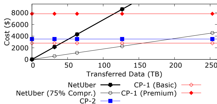
Figure 4.5: Monthly Fee for 10 GbE Flat Connectivity
