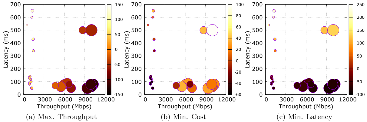
Figure 7.5: Évora policies considering three attributes with prominence to one of the three attributes. The radius of the circles represents the cost.
