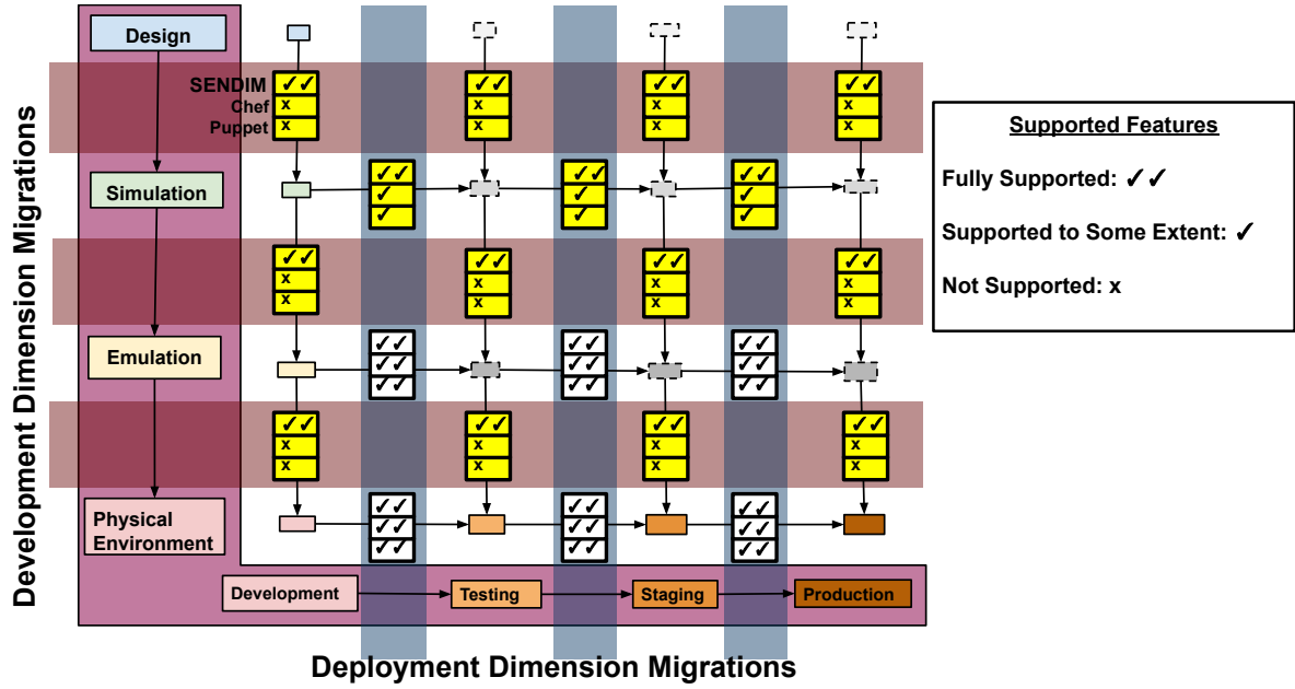
Figure 3.8: Comparative Qualitative Assessment with Configuration Management Systems
