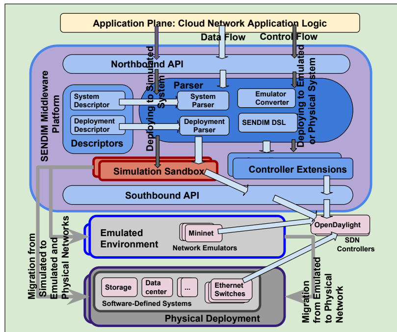
Figure 3.3: SENDIM Architecture and Deployments
