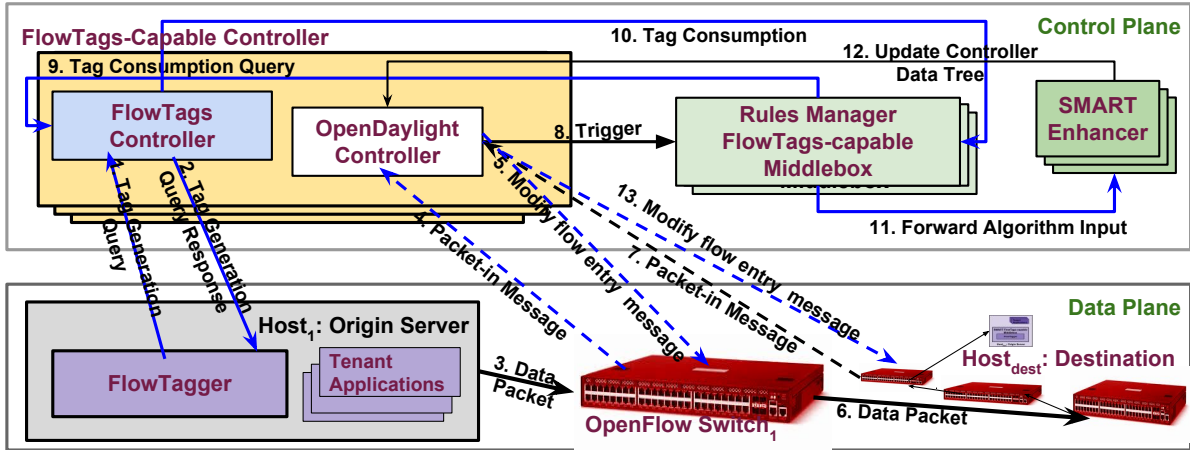
Figure 5.4: SMART Deployment and Execution
