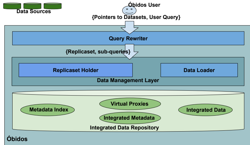
Figure 9.1: Óbidos Architecture
