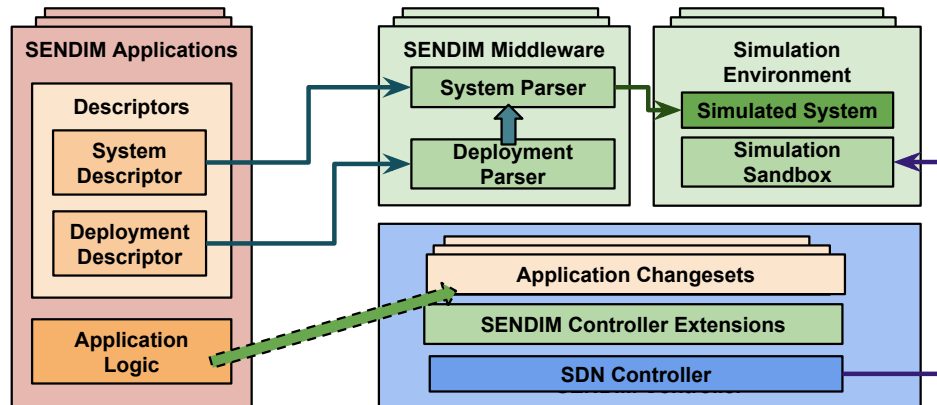
Figure 3.2: SENDIM Middleware and Applications
