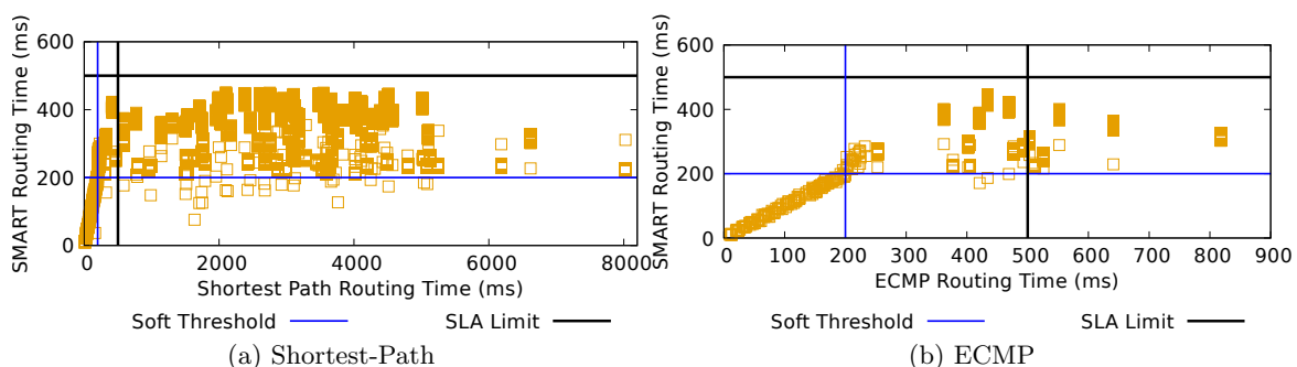
Figure 5.5: Adaptive Clone/Replicate: SMART Enhancements vs. Base Algorithm
