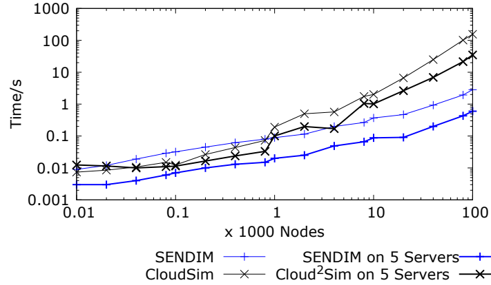
Figure 3.4: Simulating a random routing across a data center network
