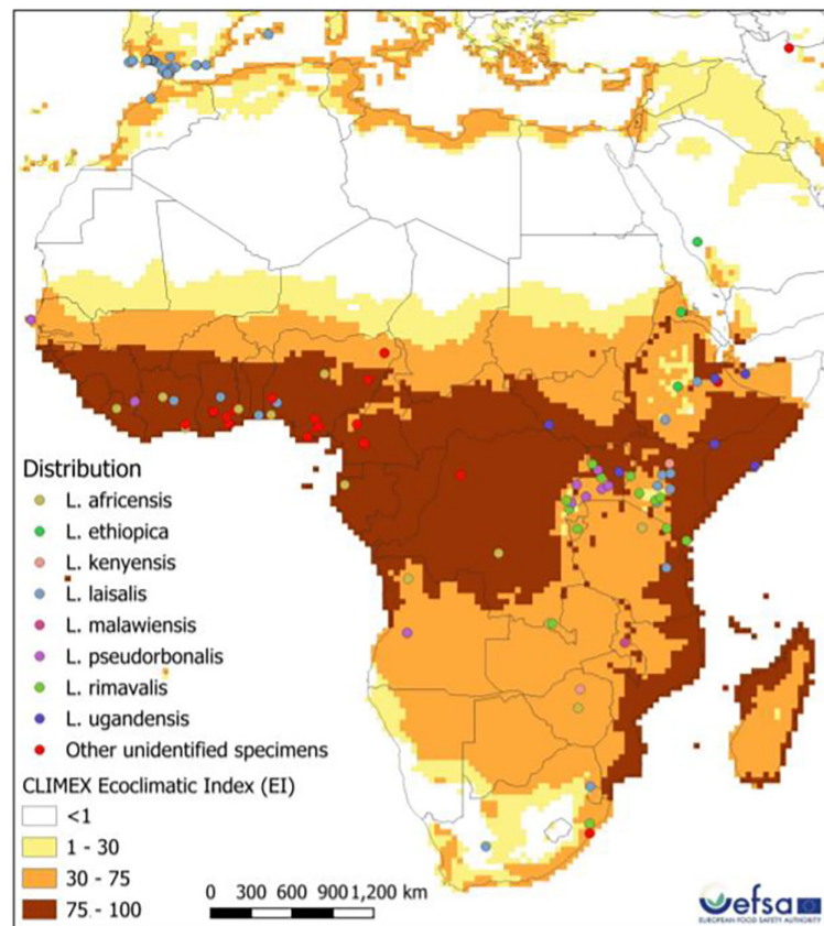
FIGURE 7 CLIMEX projection for Africa, showing four categories of Ecoclimatic index. Darker shades of yellow/brown indicate regions that are more climatically suitable for long-term survival of Leucinodes species. The CLIMEX model was parameterised for L. orbonalis using presence observations of this species in Asia, and is here used to predict independent data for African Leucinodes species in Africa.
