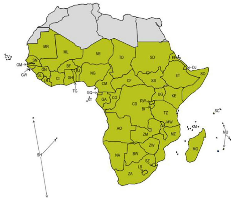
FIGURE C.4 Map of Africa indicating sub-Saharan countries (©Eurostat) that are considered as possible sources of African Leucinodes species.
