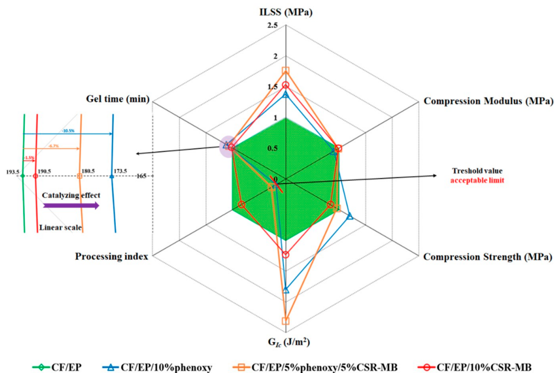
Figure 13. Spider chart summarizing (i) the processability of neat and modified EP (processing index is empirically defined as \log \eta \cdot EP / \log \eta \cdot at 110 °C with \eta \cdot in Pa·s) and (ii) the main mechanical properties of neat EP and toughened epoxy-based composites.
