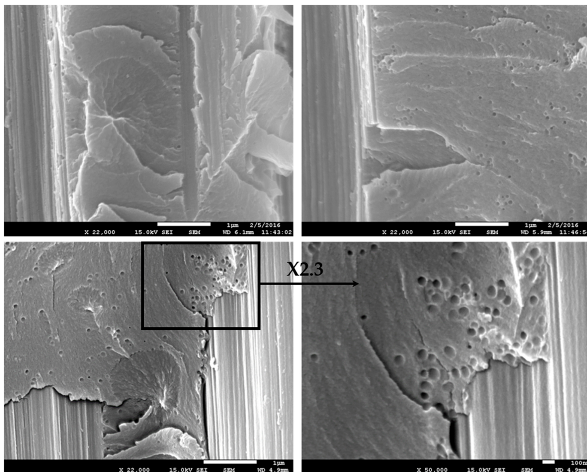
Figure 12. SEM micrographs of DCB failure surfaces of 5 wt% phenoxy/5 wt% CSR-MB epoxy-modified composite.
