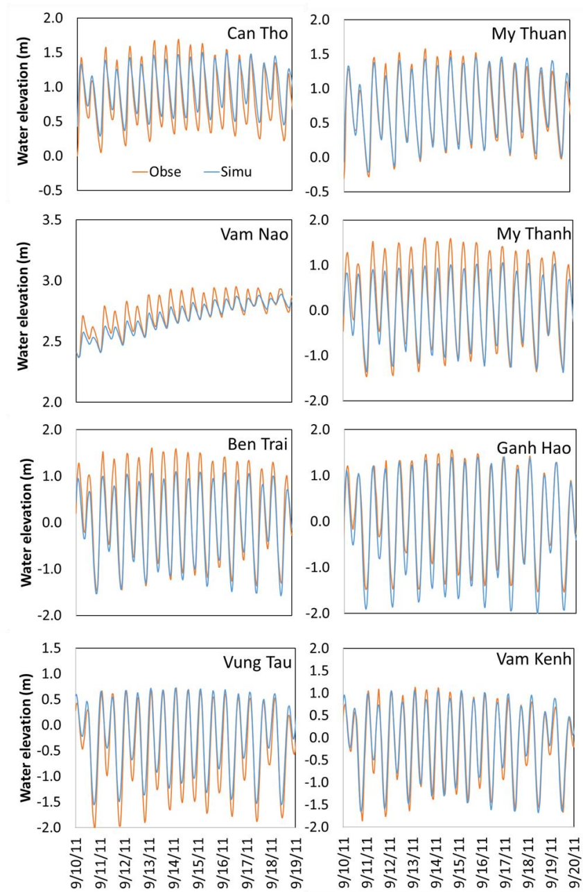
Fig. 4.7. Model calibration. The red lines present the measured data and the blue lines present the simulated one.
