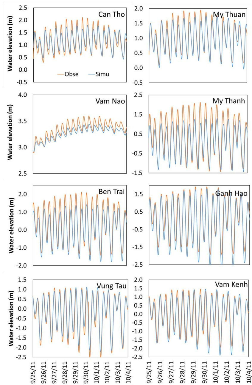
Fig. 4.8. Model validation. The red lines present the measured data and the blue lines present the simulated one.
