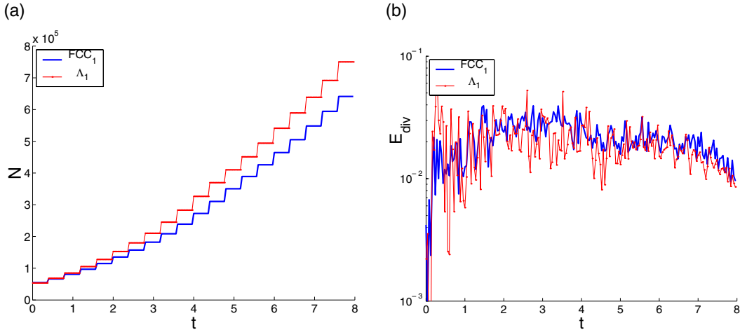
Figure 2. Re = 250 : number of particles and divergence error.
