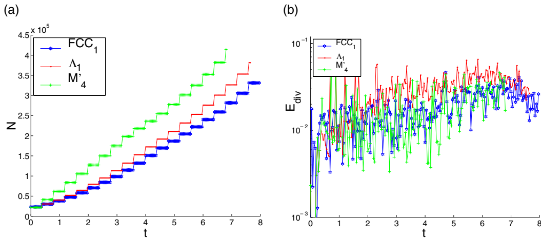
Figure 3. Re = 500 : number of particles and divergence error.
