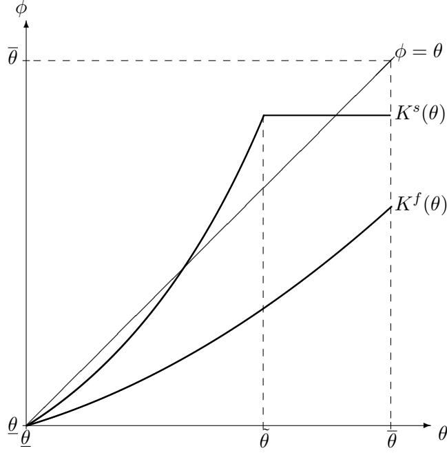
Figure 2: The entry levels under complete and incomplete information for f(\theta) = \frac{1}{\Delta} .
