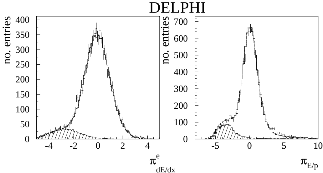
Figure 4: The \Pi_{dE/dx}^e and \Pi_{E/p} variables after application of all the other selection cuts except the one shown for 1994 data. The crosses are the data, the solid histogram is the sum of the signal and background and the shaded area is the background from \tau \not\rightarrow e\nu\bar{\nu} events.
