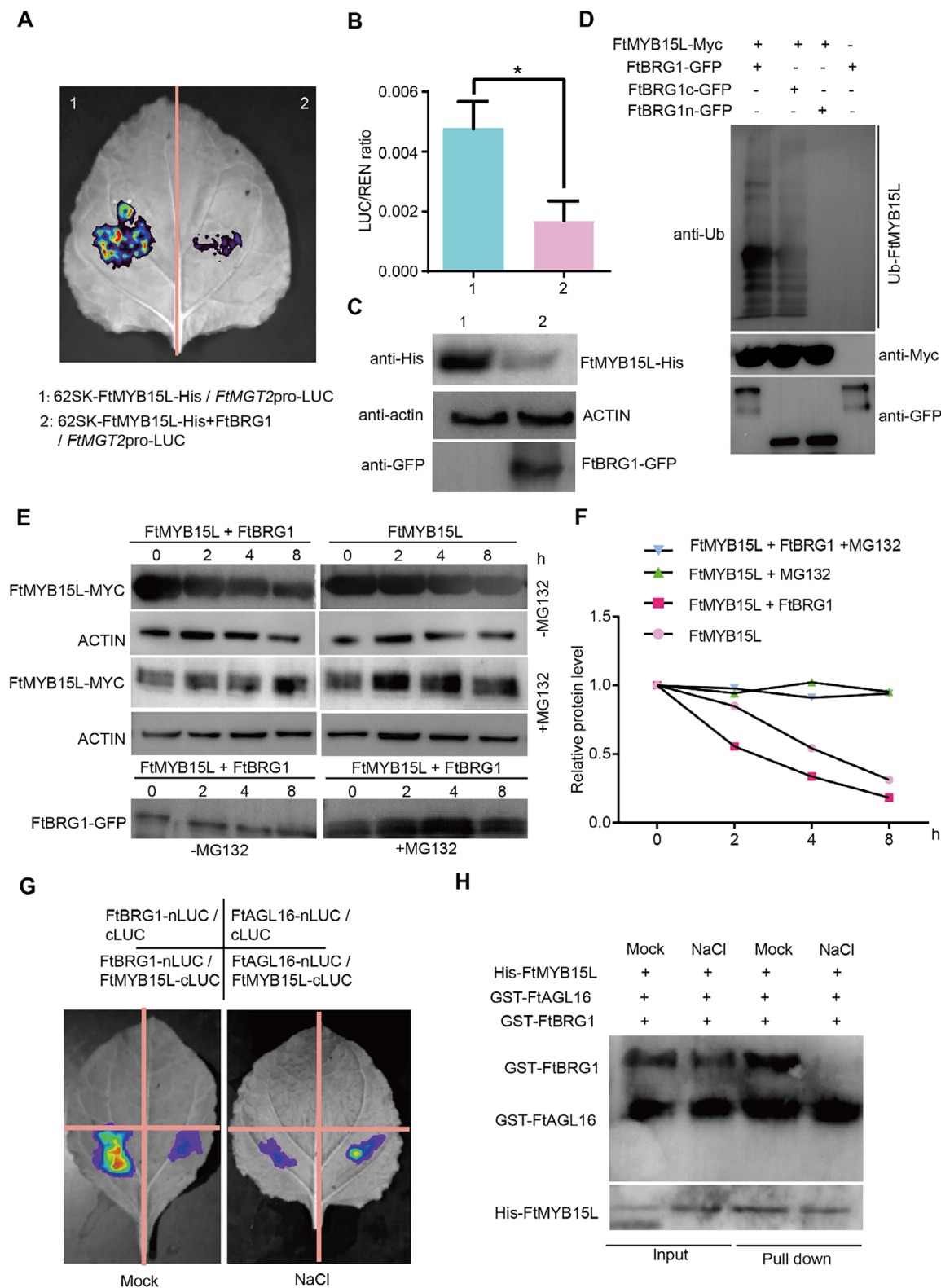
Figure 7. The FtBRG1 interacts with FtMYB15L and induces ubiquitination, thereby modulating the regulatory mechanisms of FtMGT2 . A,B) FtMGT2 prominiLUC was co-injected with 62SK-FtMYB15L-His and 62SK-FtMYB15L-His+FtBRG1 for LUC fluorescence. Data are presented as the mean \pm SD from n = 3 independent biological replicates. Statistical significance was determined using a two-sided Student's t -test. Asterisks indicate significant differences ( *P < 0.05 ). C) Immunoblotting results of FtMYB15L and FtBRG1 by transient transformed N. benthamiana leaves in (a), anti-ub, ubiquitin antibody; anti-Myc, anti Myc mouse antibody. anti-GFP, anti GFP mouse antibody. D) Ubiquitination results of FtMYB15L and FtBRG1 by transient transformed
