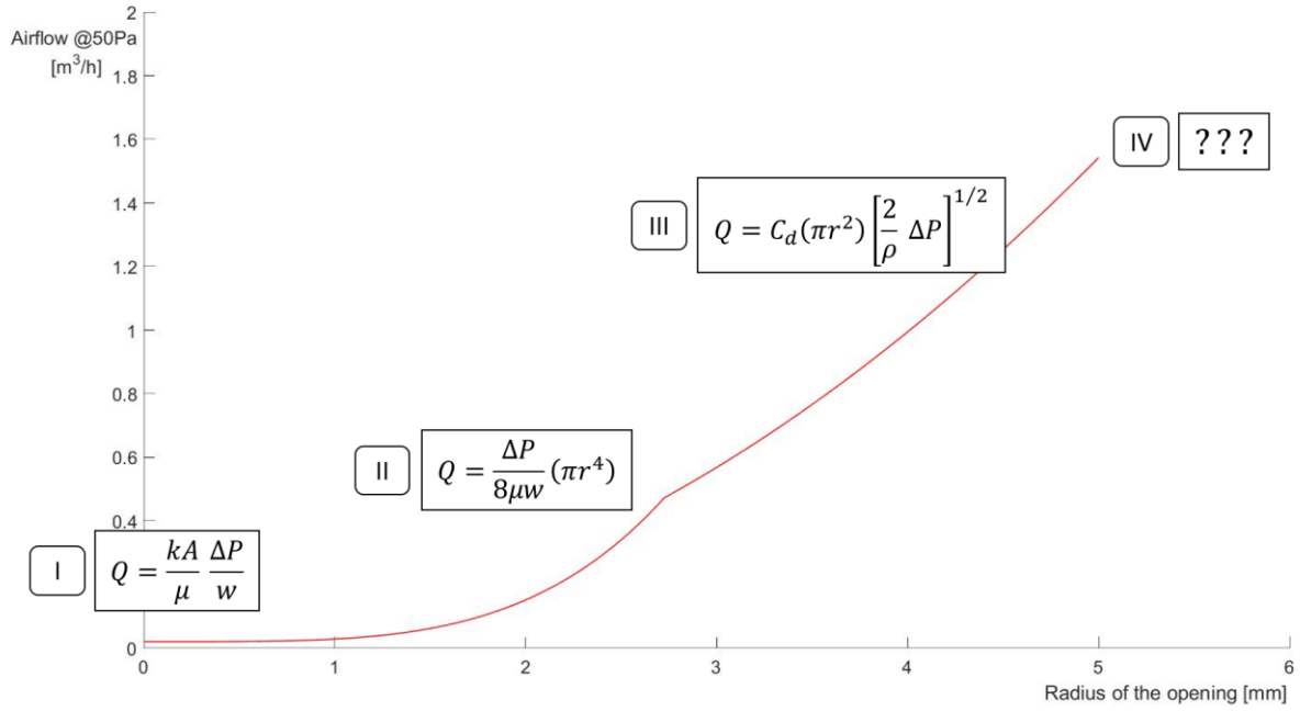
Figure 1: PIG chart for the case of a circular opening in an infinite plate
