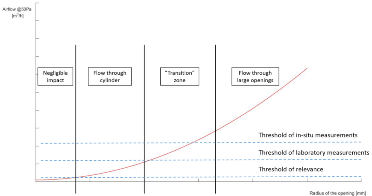
Figure 2: Smooth PIG chart with transition zone
