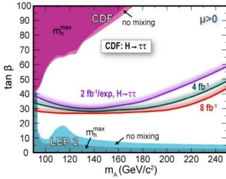
Fig. 5.5.29: The observed 95% CL limits in the tau channel in the (m_A, \tan \beta) plane, for the m_{H\text{-max}} MSSM benchmark scenario and also the no-mixing benchmark scenario, using 310 \text{ pb}^{-1} of CDF data. Projections are shown for the expected combined CDF+DØ exclusion reach for 2, 4, and 8 \text{ fb}^{-1} per experiment.
