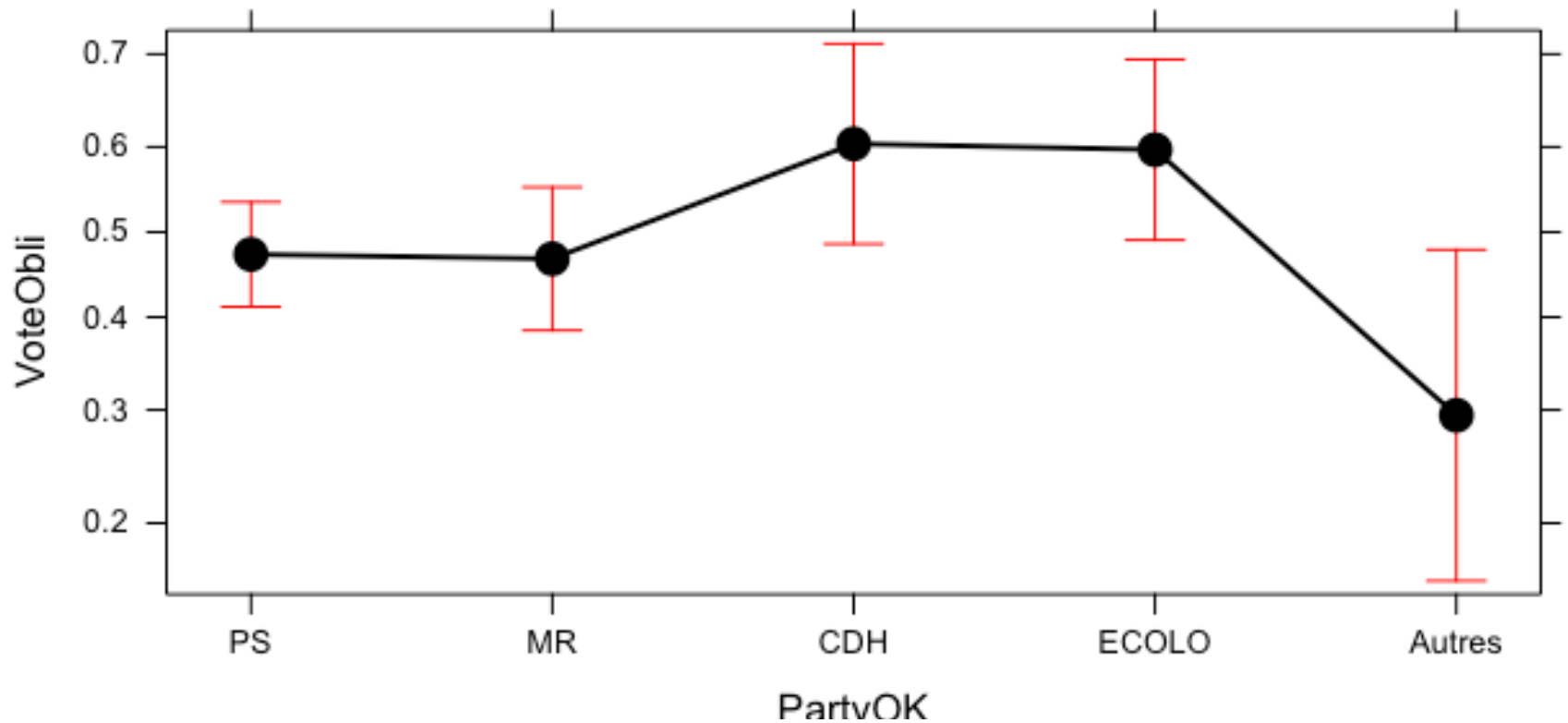
PartyOK effect plot
