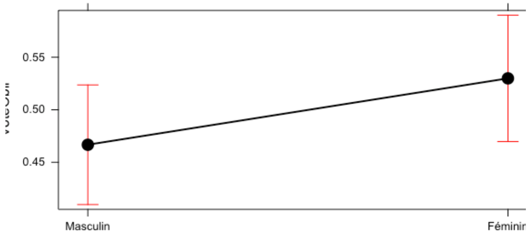
V1 effect plot
