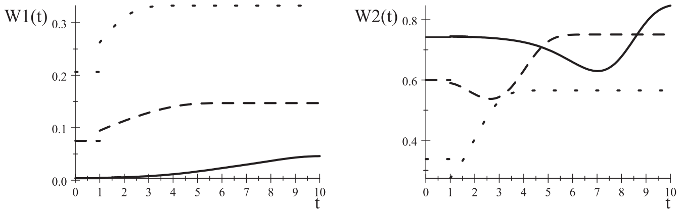
FIGURE 6 Evolution over time of welfare functions W_1(t) and W_2(t)
