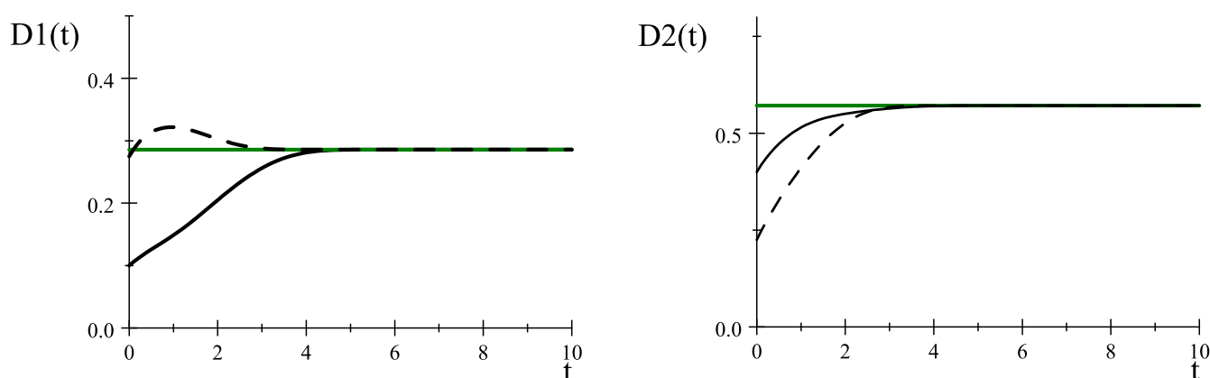
FIGURE 4 Dynamic evolution of equilibrium demand D_1(t) (left graph) and D_2(t) (right graph) [Color figure can be viewed at wileyonlinelibrary.com ]
