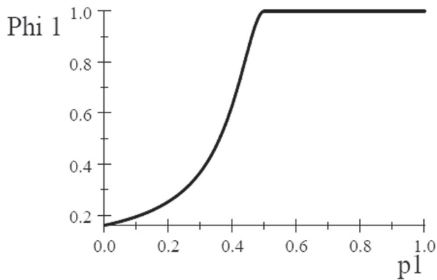
FIGURE A1 Cumulative distribution function \Phi_1(p_1) for u = 1, U_1 = 0.5, I = 0.2 , and U_2 = 0.3
