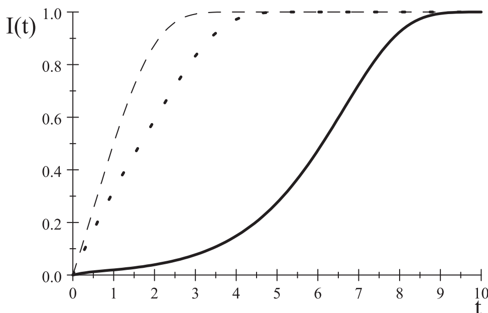
FIGURE 1 Dynamics of I(t)
