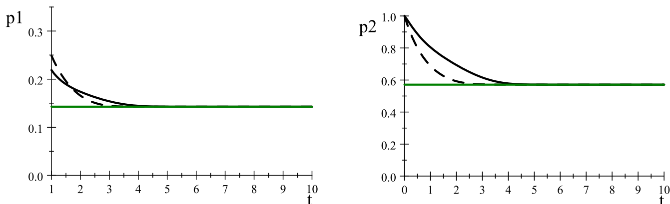
FIGURE 3 Dynamic evolution of equilibrium prices p_1(t) (left graph) and p_2(t) (right graph) [Color figure can be viewed at wileyonlinelibrary.com ]
