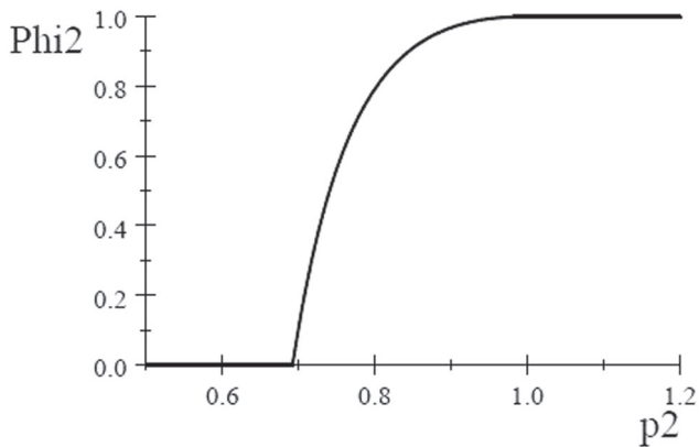
FIGURE A2 Cumulative distribution function \Phi_2(p_2) for u = 1, U_1 = 0.5, I = 0.2 , and U_2 = 0.3
