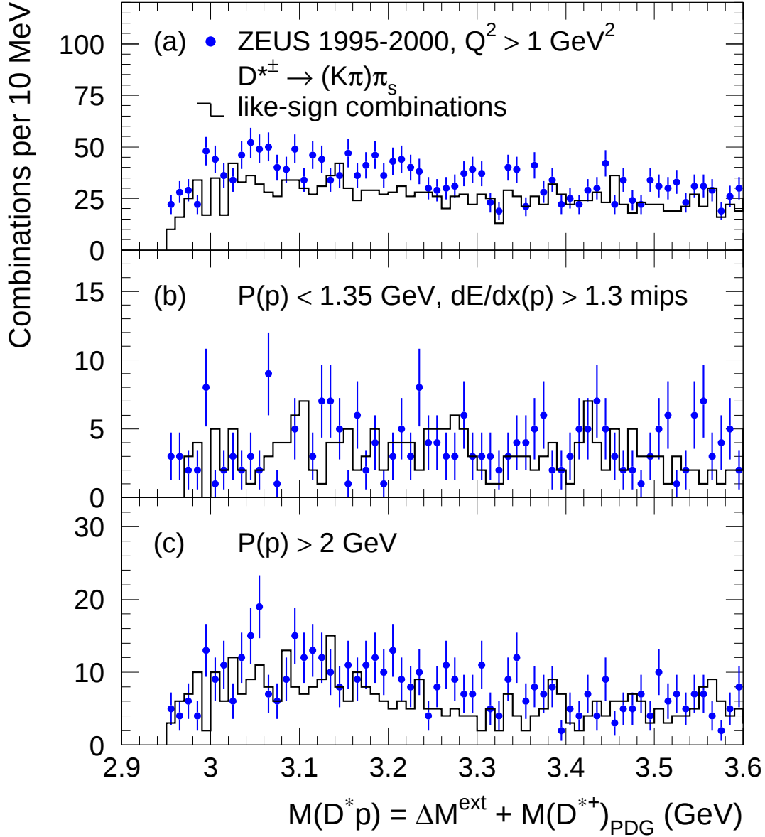
Figure 4: The distribution of M(D^*p) = \Delta M^{\text{ext}} + M(D^{*+})_{\text{PDG}} for charmed pentaquark candidates (dots) obtained in DIS with Q^2 > 1 \text{ GeV}^2 using (a) all proton candidates, (b) proton candidates with momentum below 1.35 GeV and dE/dx above 1.3 mips, and (c) proton candidates with momentum above 2 GeV. The extended mass difference is defined as \Delta M^{\text{ext}} = M(K\pi\pi_s p) - M(K\pi\pi_s) and M(D^{*+})_{\text{PDG}} is the nominal D^{*+} mass. The histograms show the M(D^*p) distributions for the like-sign combinations.
