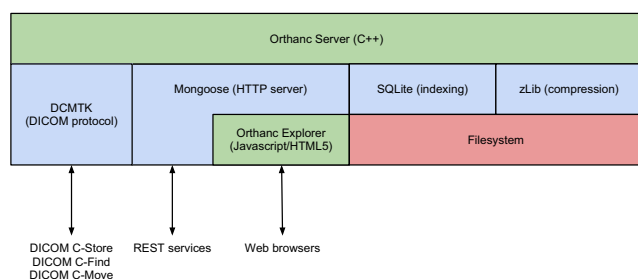
Fig. 2 The layered software architecture of the Orthanc server. The embedded third-party components are depicted in blue. Note that Orthanc can act both as a service class provider (SCP) and a service class user (SCU) for the C-Echo, C-Find, C-Store, and C-Move DICOM commands
