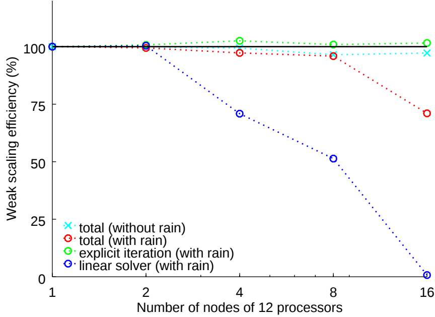
Figure 4.12: Weak scaling of the model over up to 16 \times 12 = 192 processors. The black line represents an optimal weak scaling. In the absence of a surface flow, the model weak scaling is optimal as expected from the explicit time discretization of the subsurface model. When there is a surface flow, the model overall scaling is impacted by the suboptimal scaling of the linear solver used for the implicit time discretization of the surface model. The poor scaling of the surface model is particularly clear when more than 96 processors are used.
