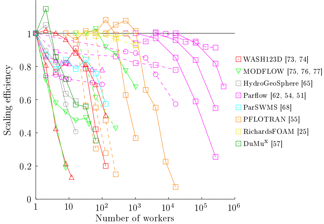
Figure 2.7: Scaling efficiency for terrestrial models. The strong scalings (continuous lines) are displayed along with the weak scalings (dashed lines), for models using the Richards equation (squares), a variant of the shallow waters (upward triangles), saturated zones only (downward triangles) or models coupling surface and subsurface (circles). The efficiency is computed based on the first data available in the series and the results are very sensible to it.
