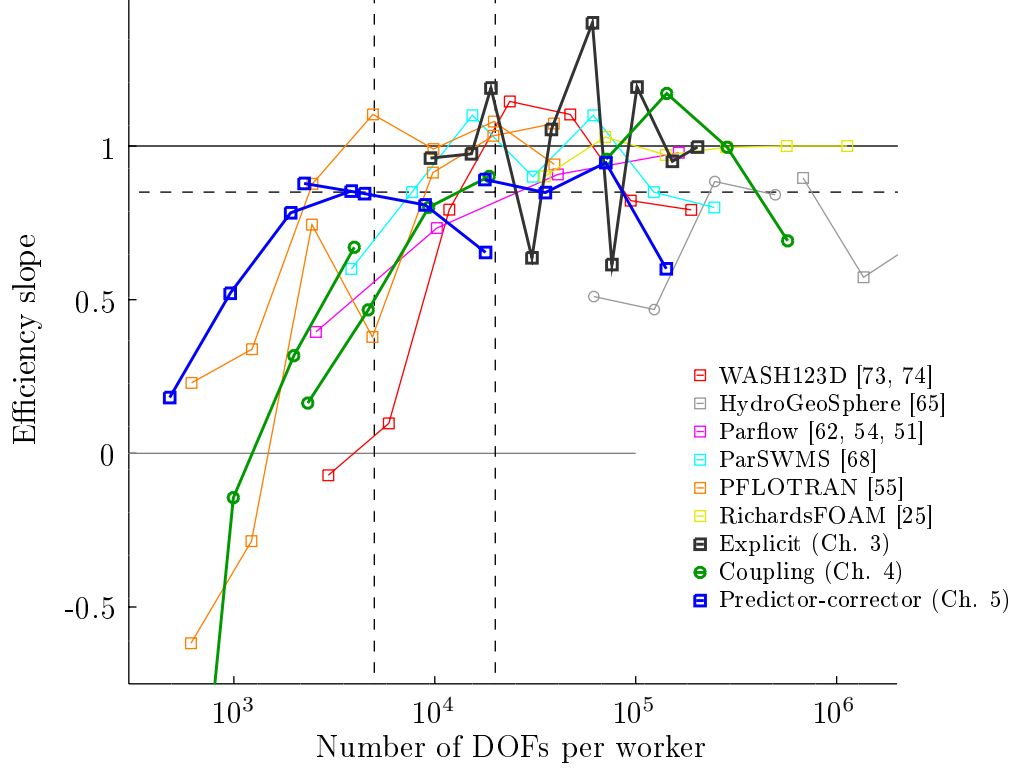
Figure 6.2: Strong scaling efficiency slopes for models of the Richards equation (squares) or models coupling surface and subsurface (circles). A slope of one represents a perfect scaling. It is expected for any model to see its performances strongly dropping under a given number of DOF/w. See Section 2.7 for more details.
