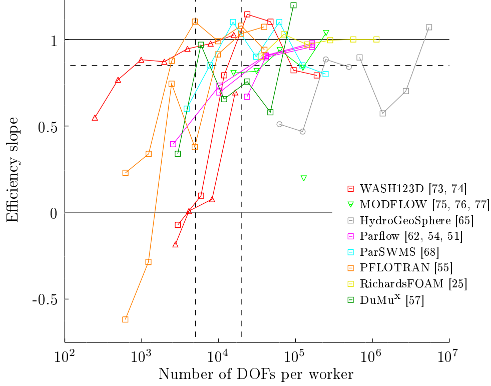
Figure 2.8: Strong scaling efficiency slopes for models of the Richards equation (squares), a variant of the shallow waters (upward triangles), saturated zones only (downward triangles) or models coupling surface and subsurface (circles). The value of one means a perfect scaling, values below zero an increase of computational time when increasing the number of workers. The dashed lines represent our limit at 0.85 to assess the scaling efficiency breakpoint and the range between 5000 to 2000 DOF/w where most models display their breakpoints.
