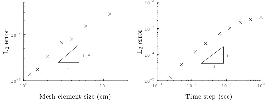
Figure 3.4: Mesh element size and time step convergence studies for the Unsaturated infiltration test-case. The L_2 norm error is computed from the finest runs (1cm for the mesh element size and 1.2510^{-3} sec for the time step).
