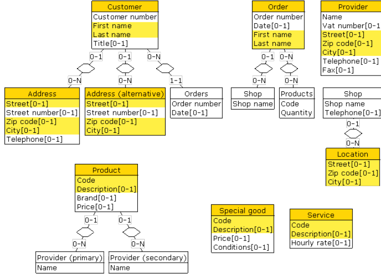
Figure 7.9: The structural redundancies within the schemas corresponding to the forms illustrated in Fig. 7.6, Fig. 7.7 and Fig. 7.8.
