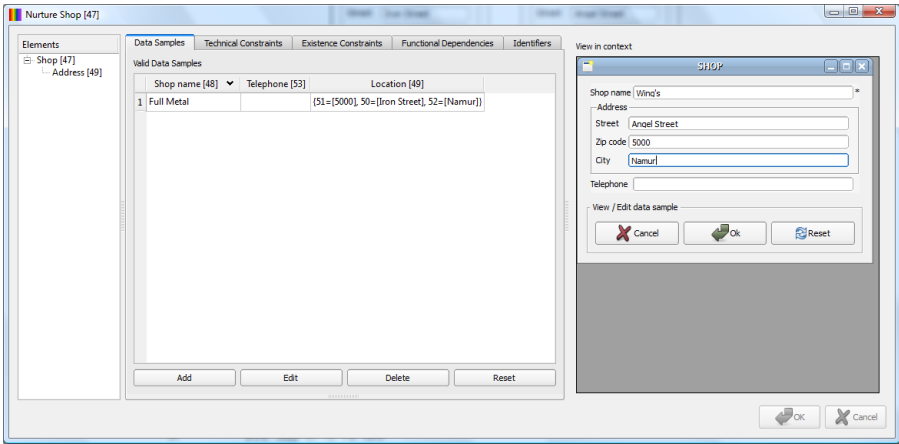
Figure 11.5: Adding data samples.
