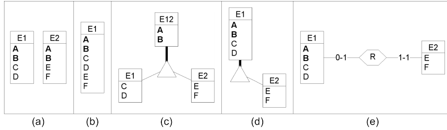
Figure 7.10: Typical cases of structural similarity.
