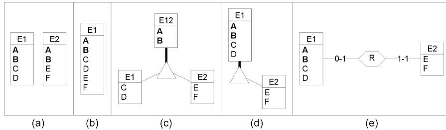
Figure 3.4: Typical cases of structural redundancies.
