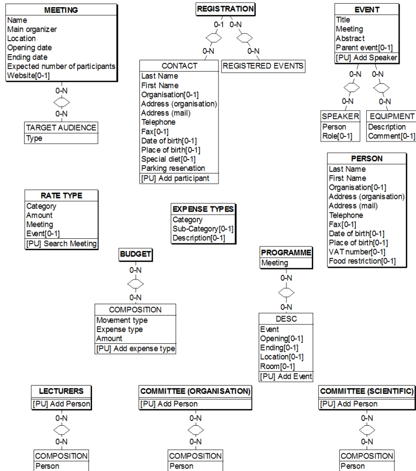
Figure 13.11: The refined schema corresponding to the raw schema of Fig. 13.10.
