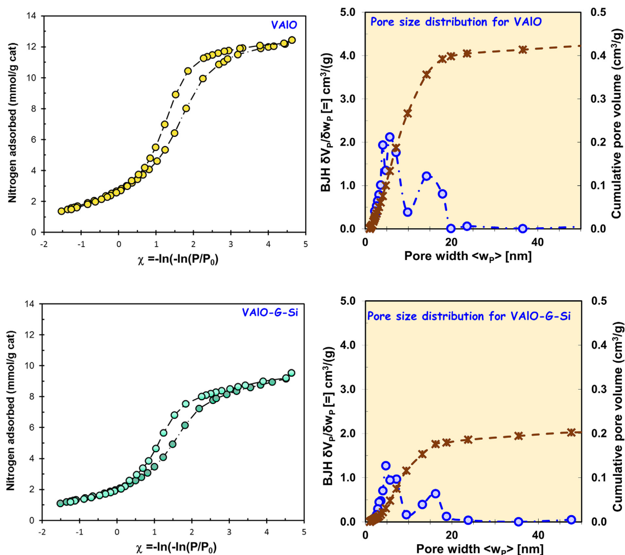
Fig. 2. Representative nitrogen physisorption isotherms, \chi -plots [35,56] for particles recovered from two representative formulations of vanadium-aluminum mixed oxide tablets: VAIO = vanadium-aluminum mixed tableted without additives. VAIO-G-Si = vanadium-aluminum mixed tableted with 1.0 wt% graphite and 5.0 wt% silica. Physisorption isotherms for the other manufactured tablets can be found in Fig. S1. Insets correspond to BJH [59] pore size distributions and cumulative pore volumes considering slit-shape pores. Other pore size distributions and cumulative pore volume plots are presented in Fig. S2.
