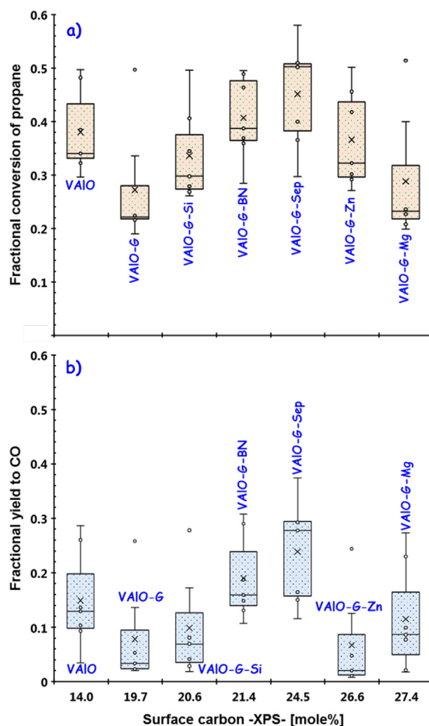
Fig. 6. Boxplots correlating the fractional conversion of propane -a)- and the molar yield to CO -b)- with the concentration of surface carbon as measured by XPS. Reaction conditions: U-shaped quartz fixed bed reactor, T = 723, 748, and 773 K, O_2/C_3H_8 molar ratios = 0.7, 1.0, 1.5, and 2.0, p = atmospheric pressure (Louvain-la-Neuve \sim 1.03 bar), catalyst weight \sim 0.1 g, average diameters of the catalyst particles 315\text{--}200 \mu\text{m} , catalytic bed volume \sim 1.0 \text{cm}^3 (catalyst plus ca. 0.4 g of quartz spheres of diameter \leq 200 \mu\text{m} ), Total gas flow, F_{\text{Tot}} [ \text{cm}^3/\text{min} ] = 40. Nomenclature: VAIO = vanadium-aluminum mixed oxide; G = 1.0 wt% graphite; Mg = magnesium oxide; Si = silica; BN = boron nitride; Zn = zinc oxide; Sep = sepiolite.
