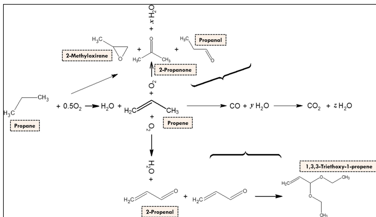
Scheme 2. Reaction scheme representing the products found during the catalytic tests. Reaction conditions: U-shaped quartz fixed bed reactor, T = 723\text{--}773\text{ K} , p = atmospheric pressure (Louvain-la-Neuve \sim 1.03 bar), catalyst weight \sim 0.1 g, average diameters of the catalyst particles 315\text{--}200\text{ }\mu\text{m} , catalytic bed volume \sim 1.0\text{ cm}^3 (catalyst plus ca. 0.4 g of quartz spheres of diameter \leq 200\text{ }\mu\text{m} ), gas flows, F_i [ \text{cm}^3/\text{min} ]: F_{\text{C}_3\text{H}_8} = 4 ; F_{\text{O}_2} = 6 ; F_{\text{N}_2} = 30 .
