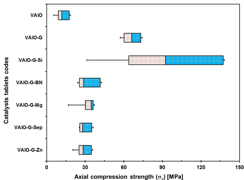
Fig. 1. Boxplots for the mechanical resistance of vanadium-aluminum mixed tablets manufactured with different shaping additives. Nomenclature: VAIO-G-Additive, where, G = 1 wt% graphite, Si = SiO 2 , BN = Boron nitride, Mg = Magnesium oxide, Sep = Sepiolite, Zn = Zinc oxide. All tablets contained 5.0 wt% of the corresponding additives.
