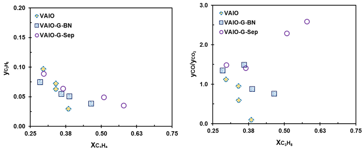
Fig. 5. Molar yield to propene ( y_{C_3H_6} ) -a)- and y_{CO}/y_{CO_2} ratio -b)- from propane oxidation as a function of the conversion of propane ( y_{C_3H_8} ) over particles recovered from tablets of the catalytic formulations: VAIO, VAIO-G-BN, and VAIO-G-Sep. Reaction conditions: U-shaped quartz fixed bed reactor, T = 723 K, p = atmospheric pressure (Louvain-la-Neuve \sim 1.03 bar), catalyst weight \sim 0.1 g, average diameters of the catalyst particles 315–200 \mu m , catalytic bed volume \sim 1.0 cm 3 (catalyst plus ca. 0.4 g of quartz spheres of diameter \leq 200 \mu m ), Total gas flow, F_{tot} [cm 3 /min] = 40. Nomenclature: VAIO = vanadium-aluminum mixed oxide; G = 1.0 wt% graphite; BN = boron nitride; Sep = sepiolite.
