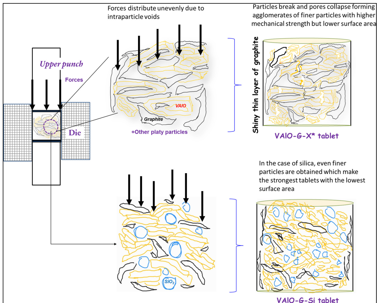
Scheme 1. Cartoon sketching the tableting production process. G = 1.0 wt% graphite; Si = 5.0 wt% silica; * = 5.0 wt% of secondary additives: MgO, boron nitride, sepiolite, and ZnO.
