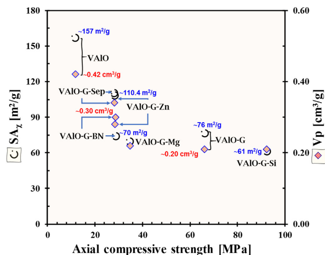
Fig. 3. Surface area, SA_x , and cumulative pore volume, V_p , plotted as a function of the median of the axial compressive strengths exhibited by the manufactured tablets. Nomenclature: VAIO-G-Additive, where, G = 1 wt% graphite, Si = SiO_2 , BN = Boron nitride, Mg = Magnesium oxide, Sep = Sepiolite, Zn = Zinc oxide. All tablets contained 5.0 wt% of the corresponding additives.
