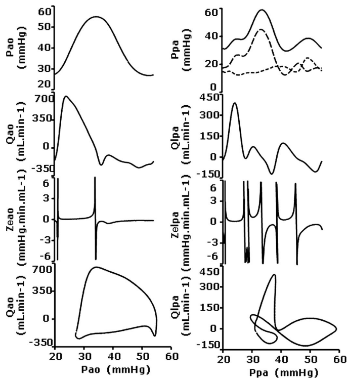
Fig. 4. Pulsatile aortopulmonary hemodynamics in the control fetuses under basal conditions. Plots correspond to population-averaged pulsatile profiles throughout the cardiac cycle along with respective P-Q hysteresis loops. P, pressure; Q, flow; Z_e , entry impedance.
