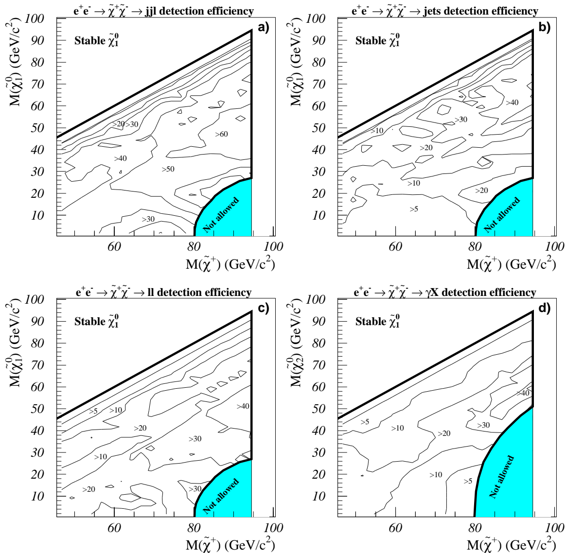
Figure 2: Chargino pair production detection efficiencies (%) for the four decay channels a) jjl , b) jets , c) ll and d) rad , at 189 GeV in the (M_{\tilde{\chi}^\pm}, M_{\tilde{\chi}^0}) plane. A stable \tilde{\chi}_1^0 is assumed. The shaded areas are disallowed in the MSSM scheme.
