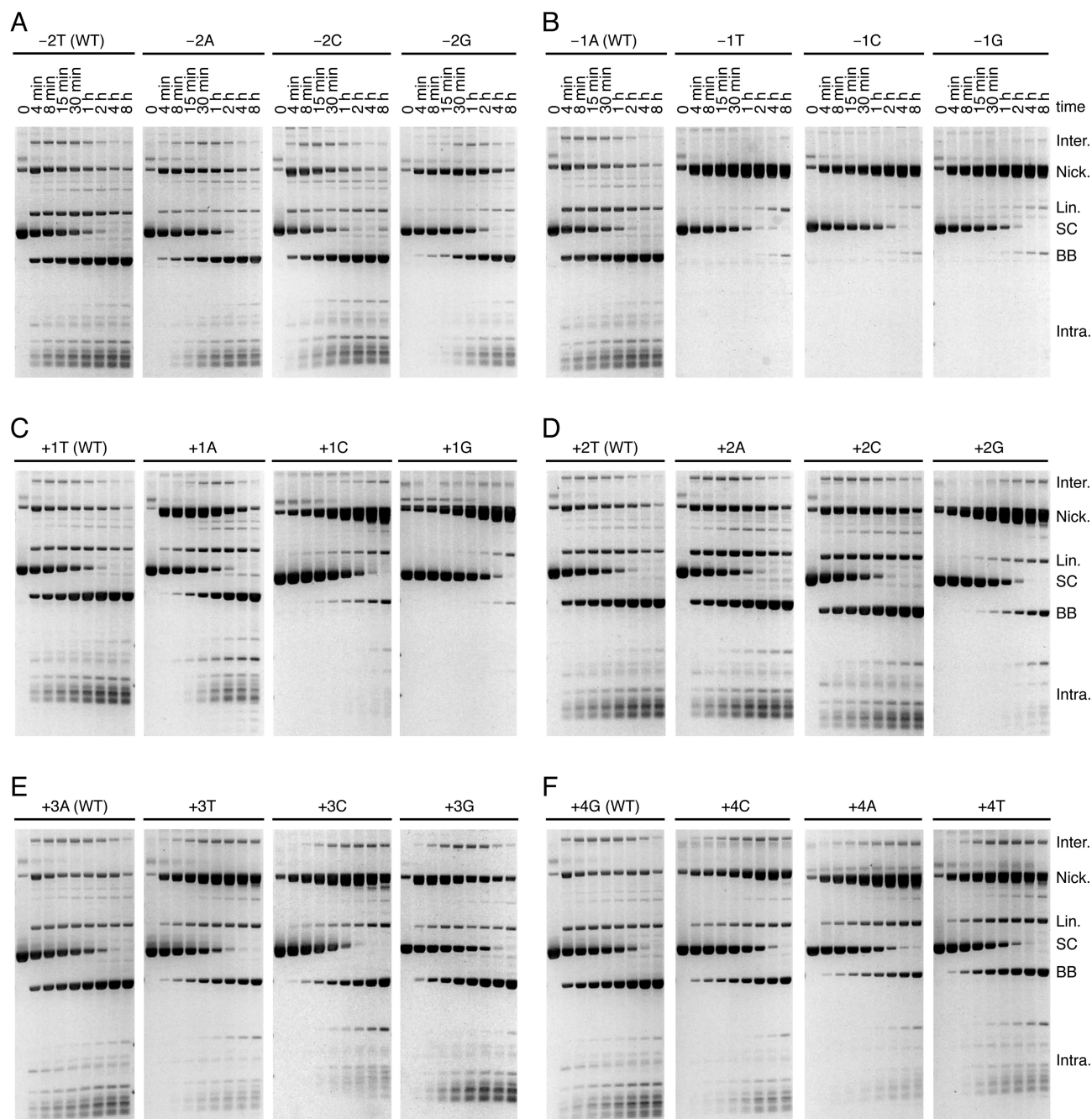
Figure 4. The effect of transposon-end mutations near the sites of cleavage. The kinetics of transposition reactions were analyzed with variants of a supercoiled transposon donor that carried symmetrical point mutations on both transposon ends. The nomenclature is as follows: negative numberings are for positions within the flanking DNA and positive numberings are for positions within the transposon end, as indicated in Figure 1C. A mutation is named after the nucleotide on the NTS. The products of the reactions are as illustrated in Figure 1A and described in the corresponding figure legend.
