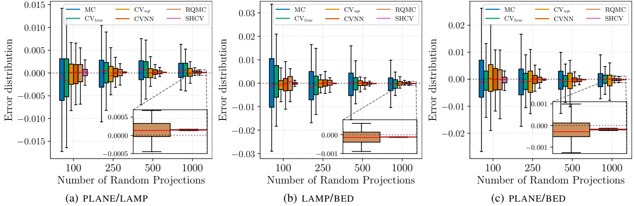
Figure 7. Boxplots of the error distribution (\widehat{SW}_n(\mu_m, \nu_m) - SW(\mu_m, \nu_m)) for different SW estimates based on n random projections with n \in \{100; 250; 500; 1000\} obtained over 100 independent runs.
