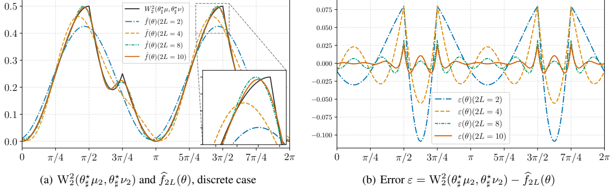
Figure 9. W_2^2(\theta_*^\mu, \theta_*^\nu) , polynomial approximation \hat{f}_{2L}(\theta) and errors \varepsilon = W_2^2(\theta_*^\mu, \theta_*^\nu) - \hat{f}_{2L}(\theta) for two discrete measures.
