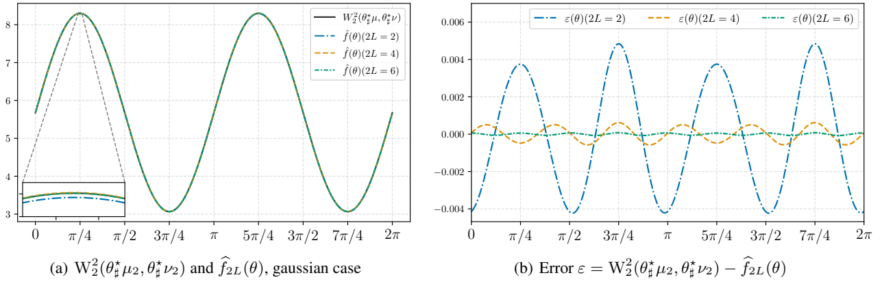
Figure 10. W_2^2(\theta_*^\mu, \theta_*^\nu) , polynomial approximation \hat{f}_{2L}(\theta) and errors \varepsilon = W_2^2(\theta_*^\mu, \theta_*^\nu) - \hat{f}_{2L}(\theta) for two Gaussian measures.
