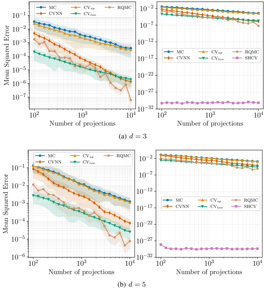
Figure 12. MSE for Gaussian distributions with proportional dispersion matrices, dimension d \in \{3, 5\} , obtained over 100 replications.
