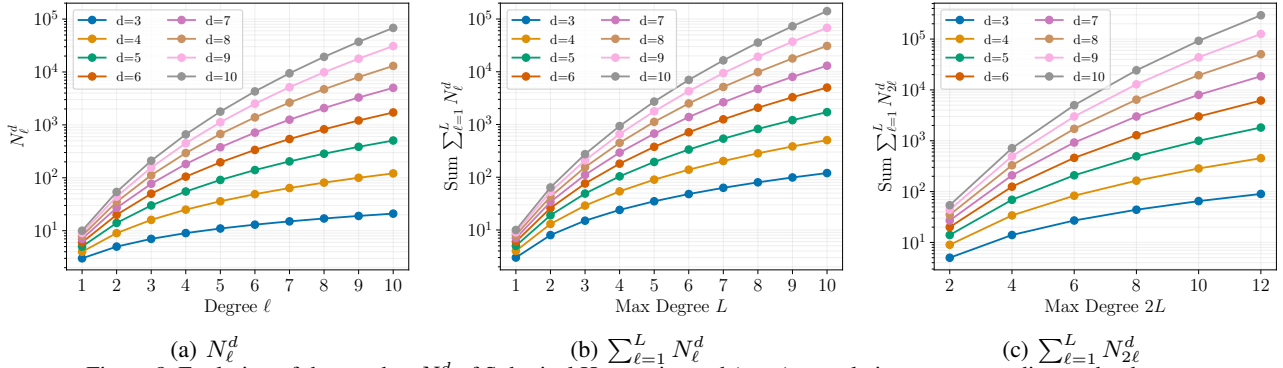
Figure 8. Evolution of the number N_\ell^d of Spherical Harmonics and (even) cumulative sums according to the degree.
