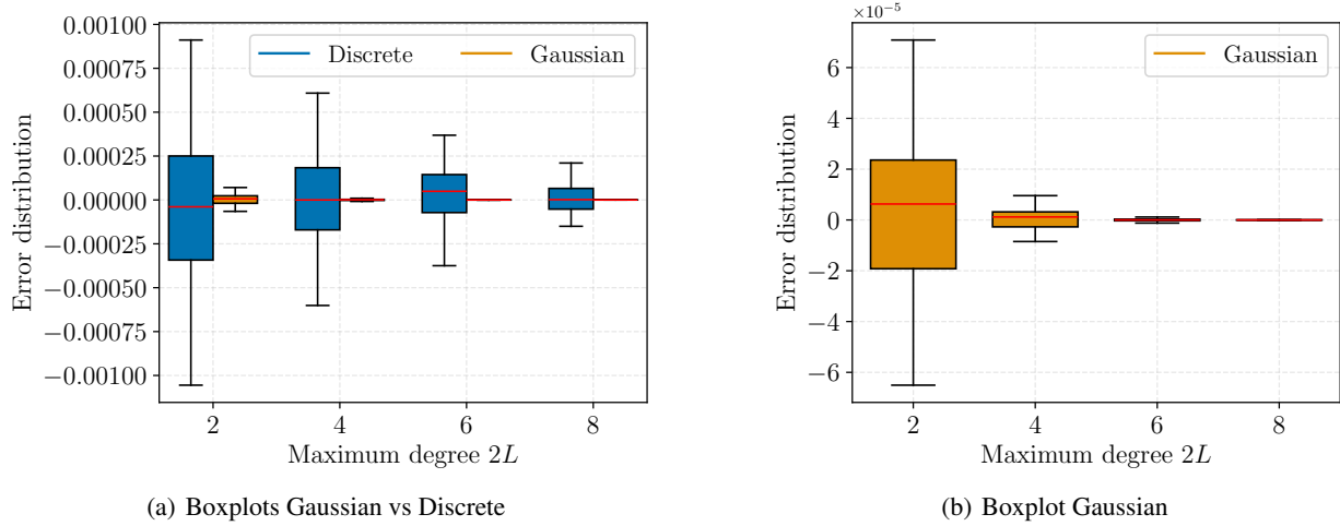
Figure 11. Error distribution of (\text{SHCV}_{n,L}^2 - \text{SW}_2^2) .
