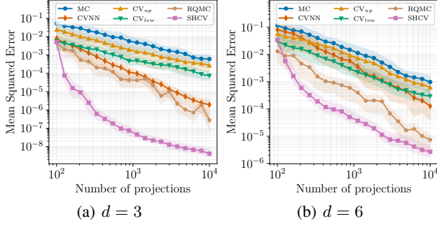
Figure 2. MSE curves for Gaussian distributions in dimension d \in \{3; 6\} based on n \in [10^2; 10^4] projections.
