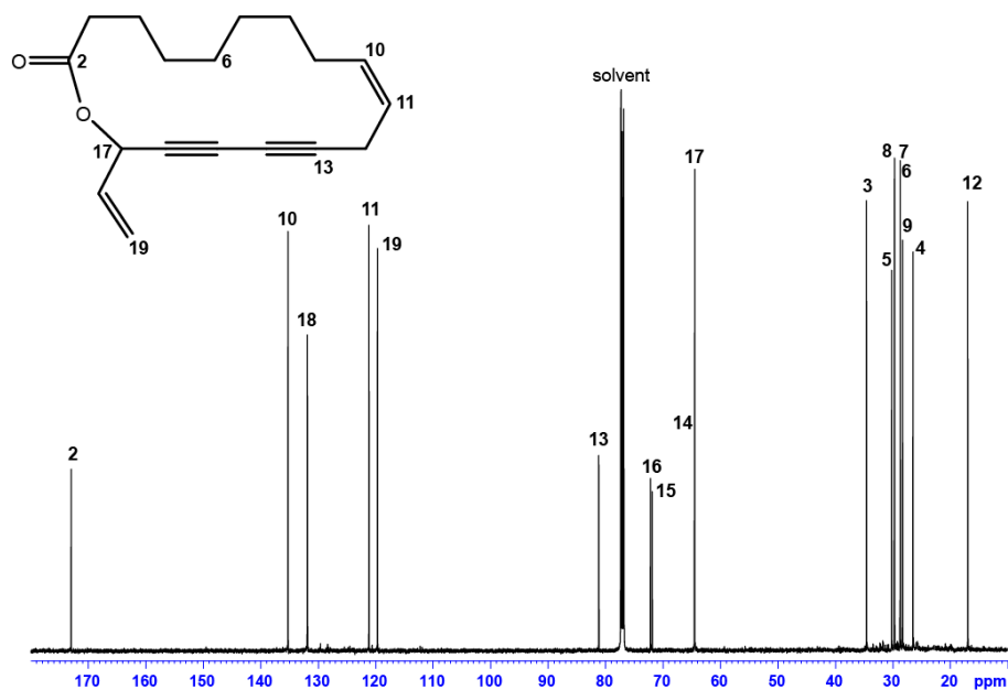
Figure 4. 13 C-NMR spectrum (125.76 MHz in CDCl 3 , 300 K) and structure (inset) of Campesterolide 33 (N.B. NMR signal assignments refer to the numbering of the molecule illustrated on the inset; the stereochemistry of 17-CH would be revealed subsequent to the VCD experiments).
