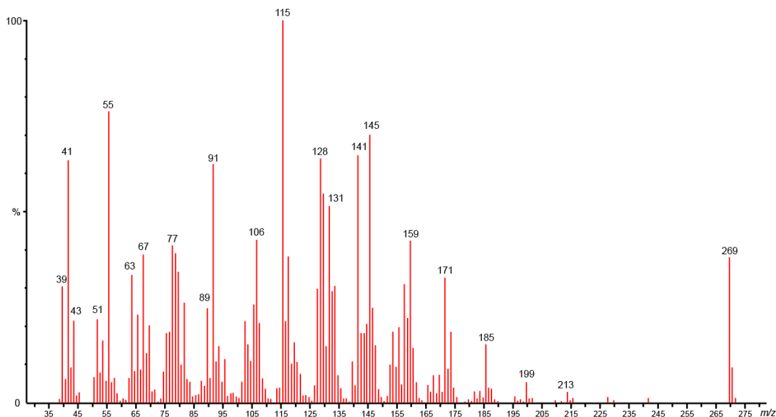
Figure 3. Electronic impact mass spectrum of campesterolide 33 (70 eV).
