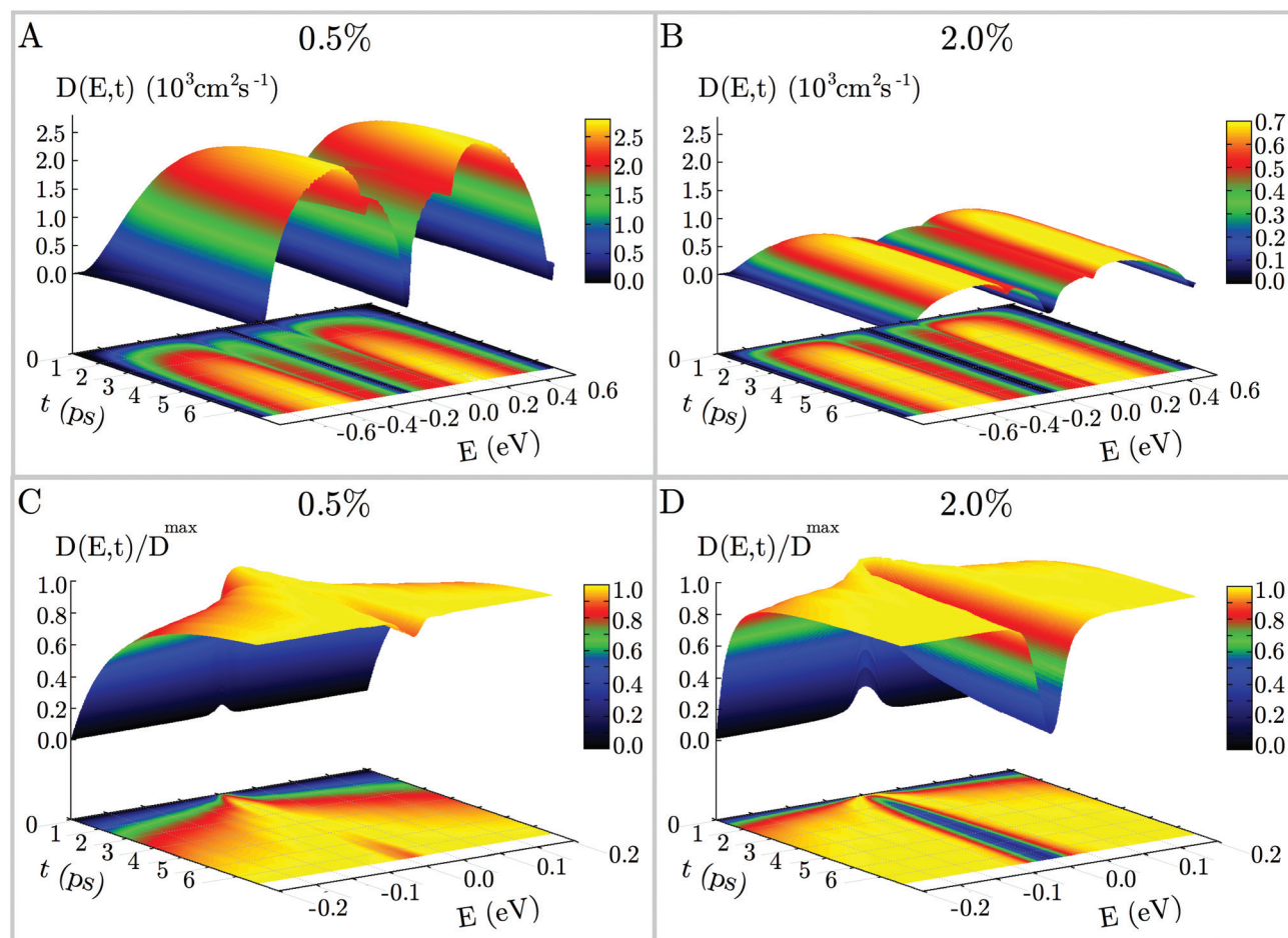
Fig. 6 3D plots of the diffusivity as a function of time and energy for 2D-C-(PP 1 ) 3 with a vacancy defect concentration of 0.5% (A) and 2.0% (B) respectively. (C) and (D) are the normalized diffusivities of (A) and (B) at a smaller energy range.
