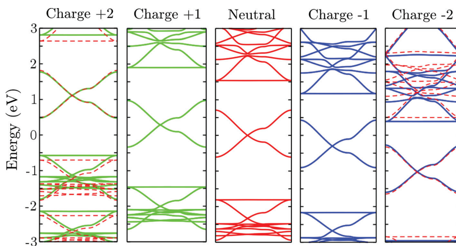
Fig. 3 Electronic band structures using the simulated doping technique coded in SIESTA for a 2D-C-(PP 1 ) 3 primitive unit cell. The Fermi energy is set to zero. The band structures of positively, neutral, and negatively charged systems are plotted with green, red, and blue lines respectively. To evidence the rigid-band approximation, the shifted neutral band structure is also reported in dashed red lines in the case of an excess charge of -2|e| and +2|e| .
