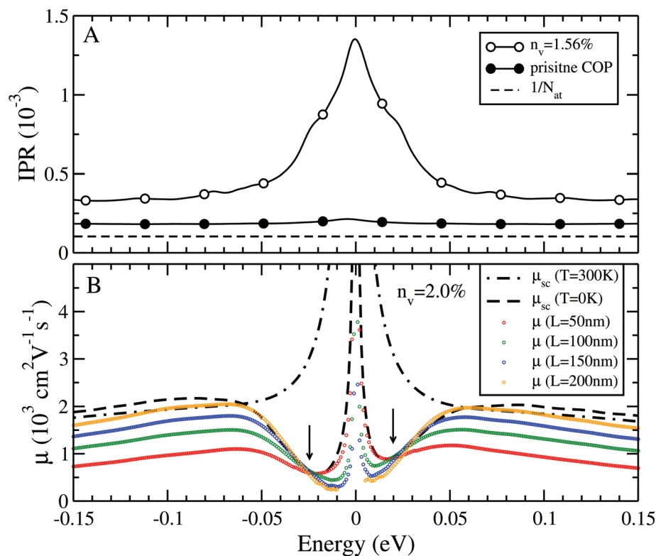
Fig. 7 (A) Inverse participation ratio (IPR) for an ideal delocalized wave function (dashed line), for a pristine (black circle), and for a 1.56% defects (white circle) 2DCP; (B) the mobilities in the semi-classical ( \mu_{sc} ) and in the quantum ( \mu ) regime for a 2DCP containing n_v = 2.0\% of randomly distributed vacancies.
