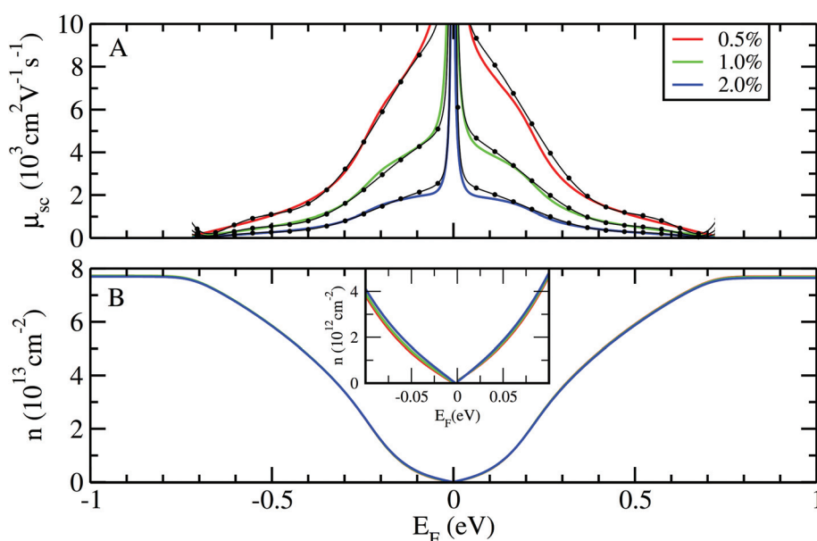
Fig. 5 (A) Charge carrier mobilities ( \mu_{sc} ) and (B) charge carrier densities ( n ) in the defective 2DCP monolayers as a function of the Fermi energy ( E_F ).
