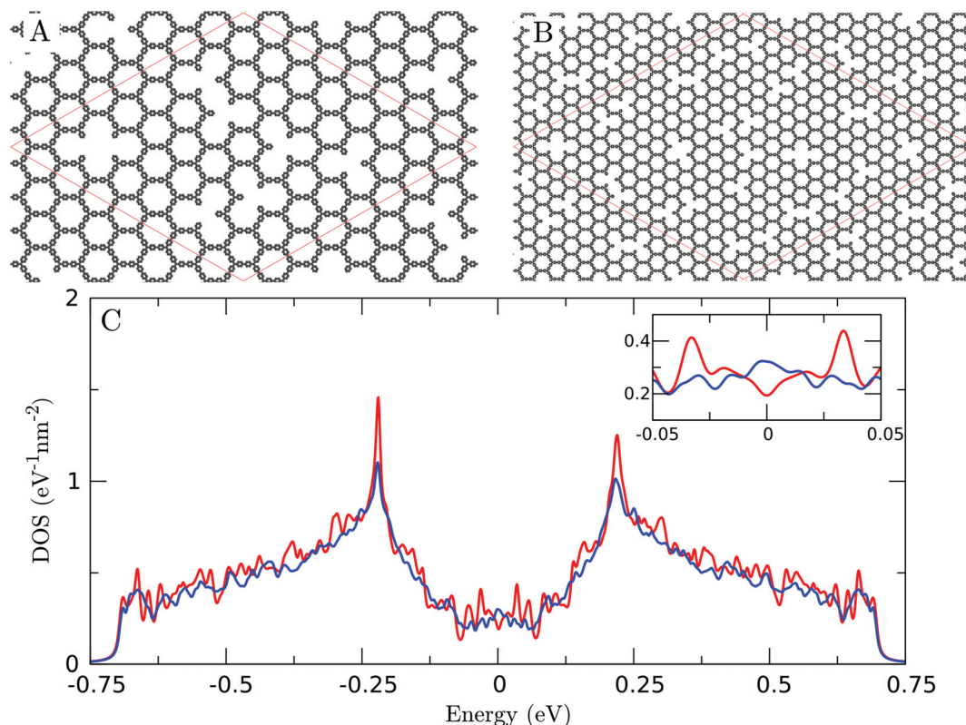
Fig. 2 (A) Atomic structures of defective 2DCP: 8 \times 8 (A) and 16 \times 16 (B) super-cell containing 6.25% of vacancies (with the same number of vacancies on each sub-lattice), (C) the respective DOS for A (red) and B (blue) (inset is a zoom in at the Fermi level).
