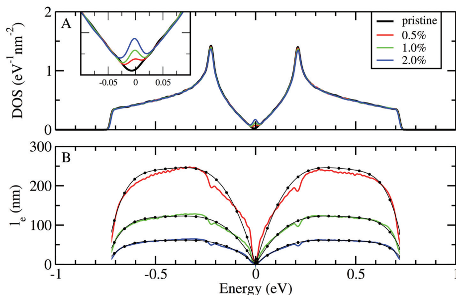
Fig. 4 (A) Densities of states of 400 \times 400 \text{ nm}^2 of a 2D-C-(PP 1 ) 3 in the pristine case and with various concentrations of vacancy defects randomly distributed (0.5%, 1.0%, 2.0%). (B) Carrier mean free paths ( l_e ) of the corresponding defective 2DCP monolayers. Black dotted lines are fits obtained following the Fermi golden rule.
