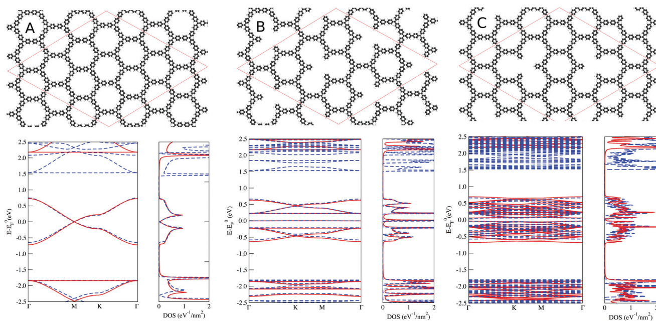
Fig. 1 Top: inside the red cell, 4 \times 4 super cells for a pristine 2DCP in (A), containing four monovacancies (12.5%) in (B) and containing two monovacancies (6.25%) with an equivalent number on both sub-lattices in (C). Bottom: ab initio (dashed blue line) and tight-binding (red thick line) band structures and densities of states (DOS) of the corresponding atomic structures (A), (B), and (C). The Fermi energy is aligned with E = 0 eV.
