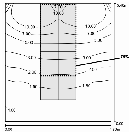
Figure 4: daylight factor levels for the “aware flexibility – level one” concept shown in Fig.3 and a 40% glazed façade. The dotted line identifies the 75% of spaces occupied for critical visual tasks.
