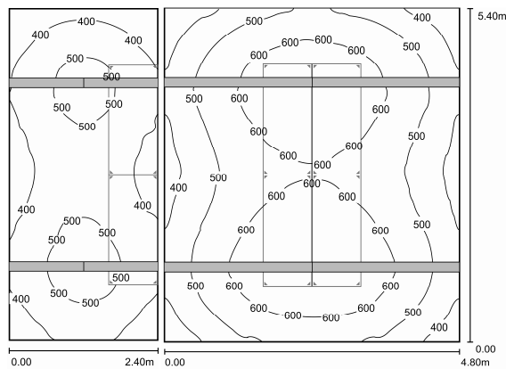
Figure 2: Dialux simulation of the artificial lighting in a full flexibility concept. Lighting devices simulated are Philips TBS340 LC 1xTL-D36W/840 CON C6. Resultant power is 13.12\text{W/m}^2 .
