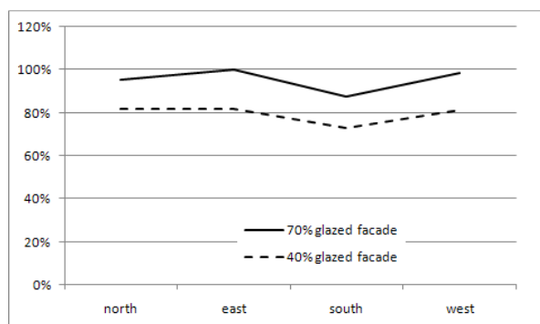
Figure 7: Relative primary energy consumption of a single office (summing heating, cooling and humidity control) as a function of orientation and façade design.
