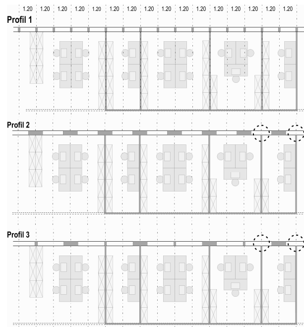
Figure 1: Confrontation of an irregular space division (full flexibility test) with 3 facade designs: fully glazed, window's array based (1 for every 2 axis) and window's array based (1 every 3 axis). For designs based on window's array, local discomfort occurs (dotted circles).
