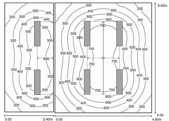
Figure 5: Dialux simulation of the artificial lighting in an aware flexibility concept – level one. Lighting devices simulated are Zumtobel L-FIELDS A A 2/28W. Resultant power is 9.46 W/m 2 .
