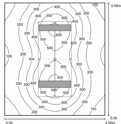
Figure 6: Dialux simulation of the artificial lighting in an aware flexibility concept – level two. Lighting devices simulated are Zumtobel L-FIELDS A A 2/35W T16. Resultant power is 5.83 W/m 2 .
