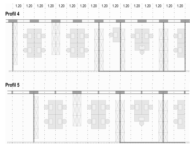
Figure 3: Examples of the aware flexibility concept: first level, on a 2 modules base (above) and second level, on a 4 modules base (under).
