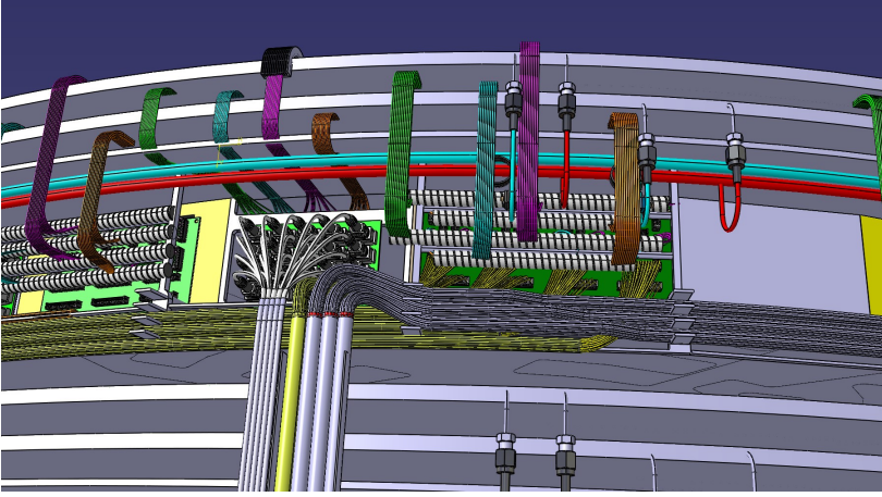
Figure 5.13. | CAD view of the PP0 region with the services included.
