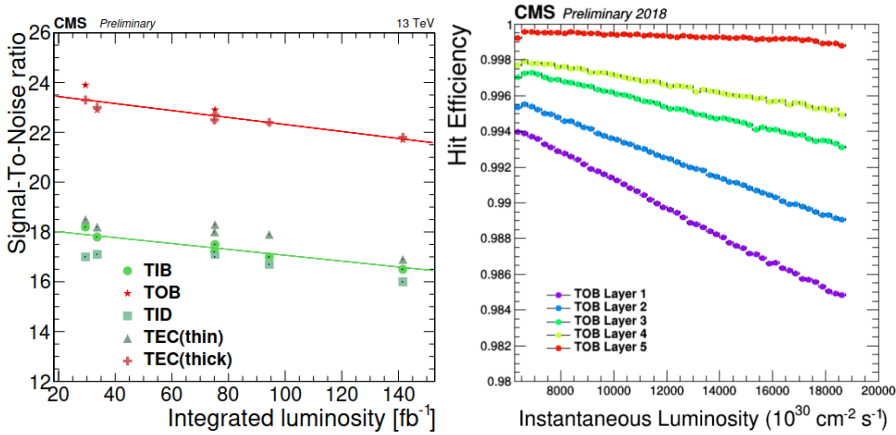
Figure 3.10. | The evolution of the run-2 S/N in the different detector partitions as a function of integrated luminosity (left) and single hit efficiencies as a function of the instantaneous luminosity, as seen during the 2018 data-taking period (right). From Ref. [47].
