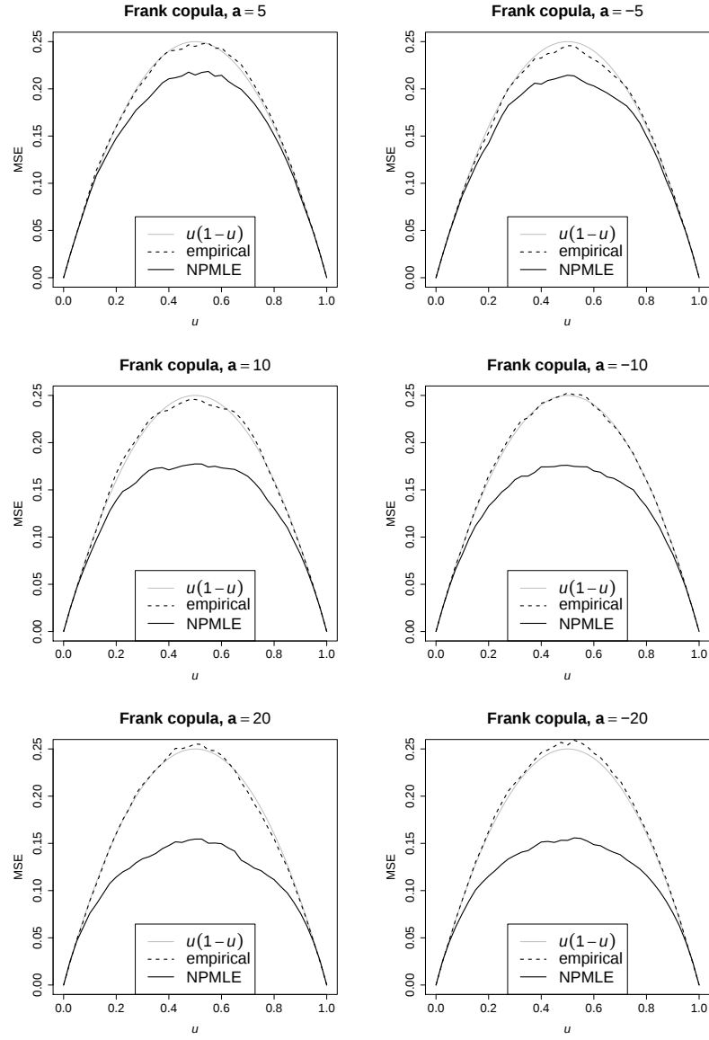
Figure 6: Estimates of the normalized mean squared error E[n\{\hat{F}_n(u) - u\}^2] based on M = 5\,000 samples of size n = 100 from the bivariate Frank copula with parameter a = -\log \theta \in \{\pm 5, \pm 10, \pm 20\} together with the function u \mapsto u(1-u) . Here \hat{F}_n is the empirical distribution function (dashed) or the nonparametric maximum likelihood estimator if the copula is known (solid).
