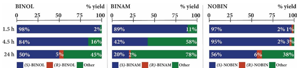
Fig. 1 Degradation of (S)-BINOL, (S)-BINAM and (S)-NOBIN under ball milling conditions: 1a , 2a (100 mg, 0.35 mmol) or 3a (50 mg, 0.18 mmol) were added to a zirconium oxide milling vessel (10 mL) with two zirconium oxide balls (diameter: 10 mm) and milled in an MM400 ball mill at 30 Hz. Percentages were determined using quantitative HPLC. 'Other' refers to species formed via cyclisation and oligomerisation.
