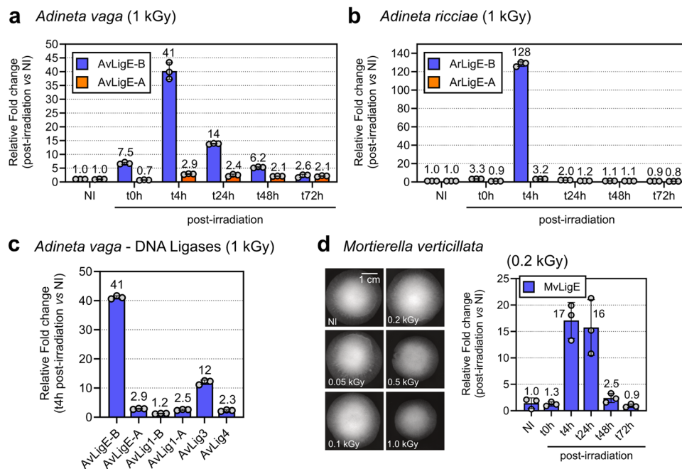
Fig. 3 | Relative mRNA expression analysis of DNA ligases upon irradiation in bdelloid species Adineta vaga and Adineta ricciae and in the fungus species Mortierella verticillata . a, b, d Kinetics expression analysis of DNA ligase E from A. vaga , A. ricciae and M. verticillata , respectively. The bdelloid rotifer species were irradiated at 1 kGy and M. verticillata at 0.2 kGy of X-ray. The mRNA level at t0h, t4h, t24h, t48h and t72h post-irradiation was determined by qPCR in triplicate. The relative expression were measured in comparison to the non-irradiated control (NI). In d the IR survival rate of M. verticillata was determined by its growth efficiency after X-ray irradiation to doses ranging from 0.05 to 1 kGy. A significant
