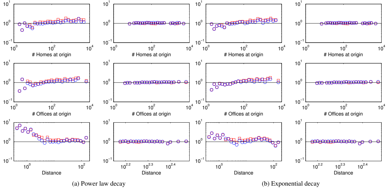
Figure 12: Plots of the prediction ratio \hat{w}_{ij}/w_{ij} for commuting distance of d < 150 km (left panels) and d_{ij} \geq 150 km (right panels) for (a) the power law decay f(d_{ij}) = d_{ij}^\gamma , and (b) the exponential decay f(d_{ij}) = e^{\gamma d_{ij}} . Red squares indicate mean values, and blue circles indicate medians.
